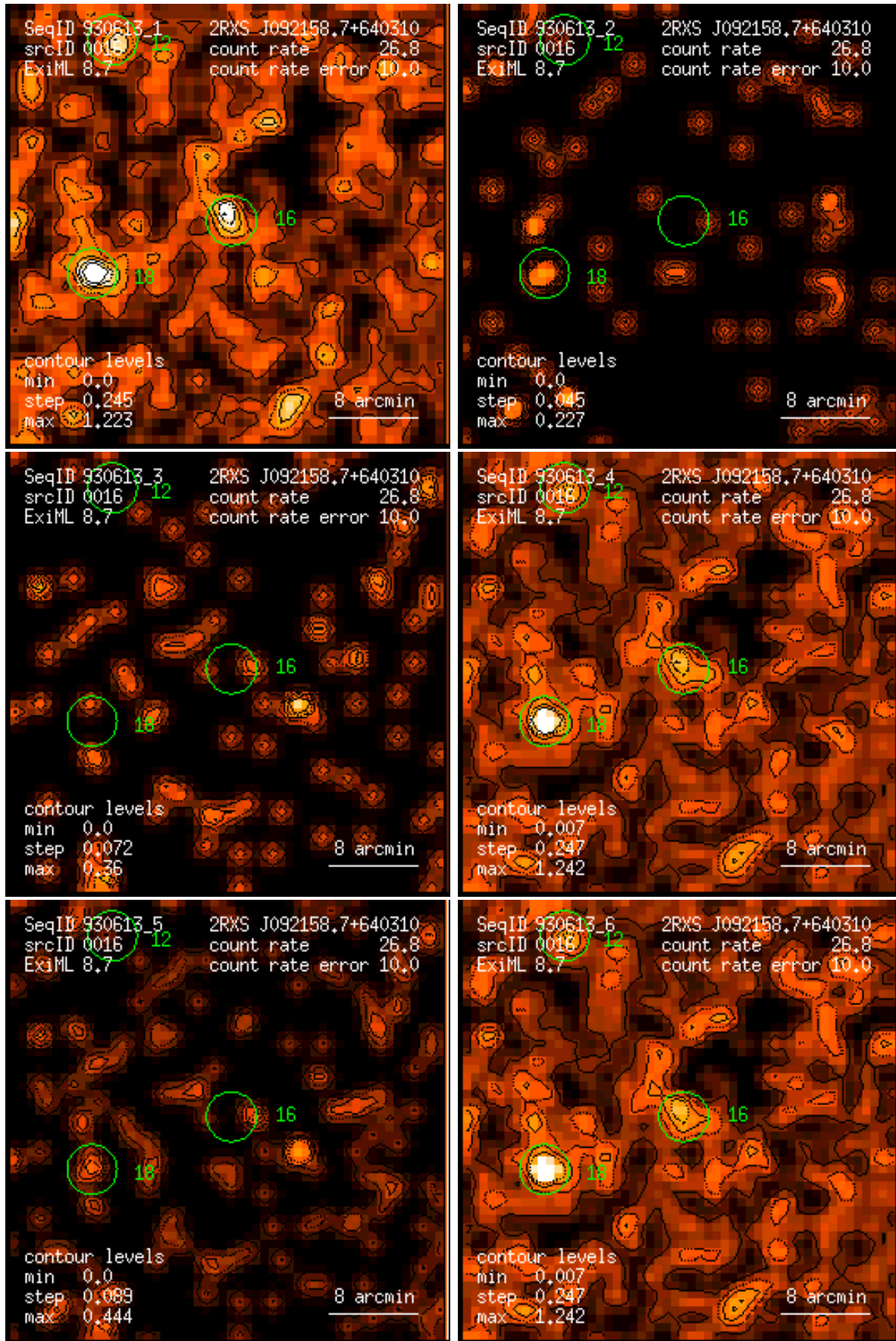
Figure 16: RASS 930613: detection 0016: band rate images, Gaussian filter: (1) PSPC channels 11 – 41, (2) 52 – 90, (3) 91 – 201, (4) 11 – 235, (5) 52 – 201, (6) 11 – 201. Broad band rates in counts/ks. Band rate contour levels in counts/ks/arcmin 2 .
