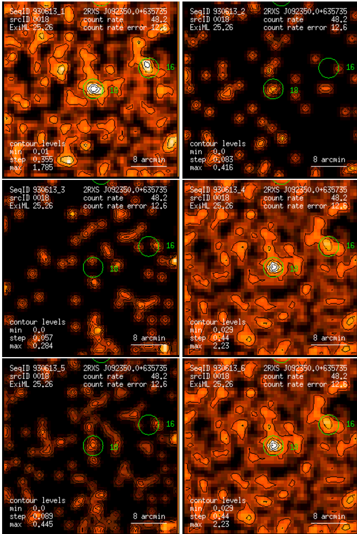
Figure 18: RASS 930613: detection 0018: band rate images, Gaussian filter: (1) PSPC channels 11 – 41, (2) 52 – 90, (3) 91 – 201, (4) 11 – 235, (5) 52 – 201, (6) 11 – 201. Broad band rates in counts/ks. Band rate contour levels in counts/ks/arcmin 2 .
