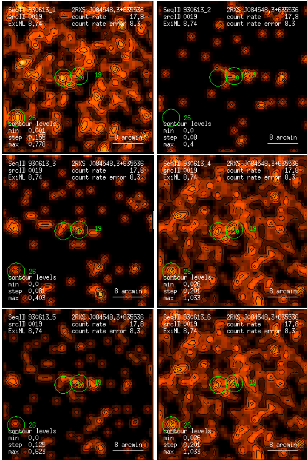
Figure 19: RASS 930613: detection 0019: band rate images, Gaussian filter: (1) PSPC channels 11 – 41, (2) 52 – 90, (3) 91 – 201, (4) 11 – 235, (5) 52 – 201, (6) 11 – 201. Broad band rates in counts/ks. Band rate contour levels in counts/ks/arcmin 2 .
