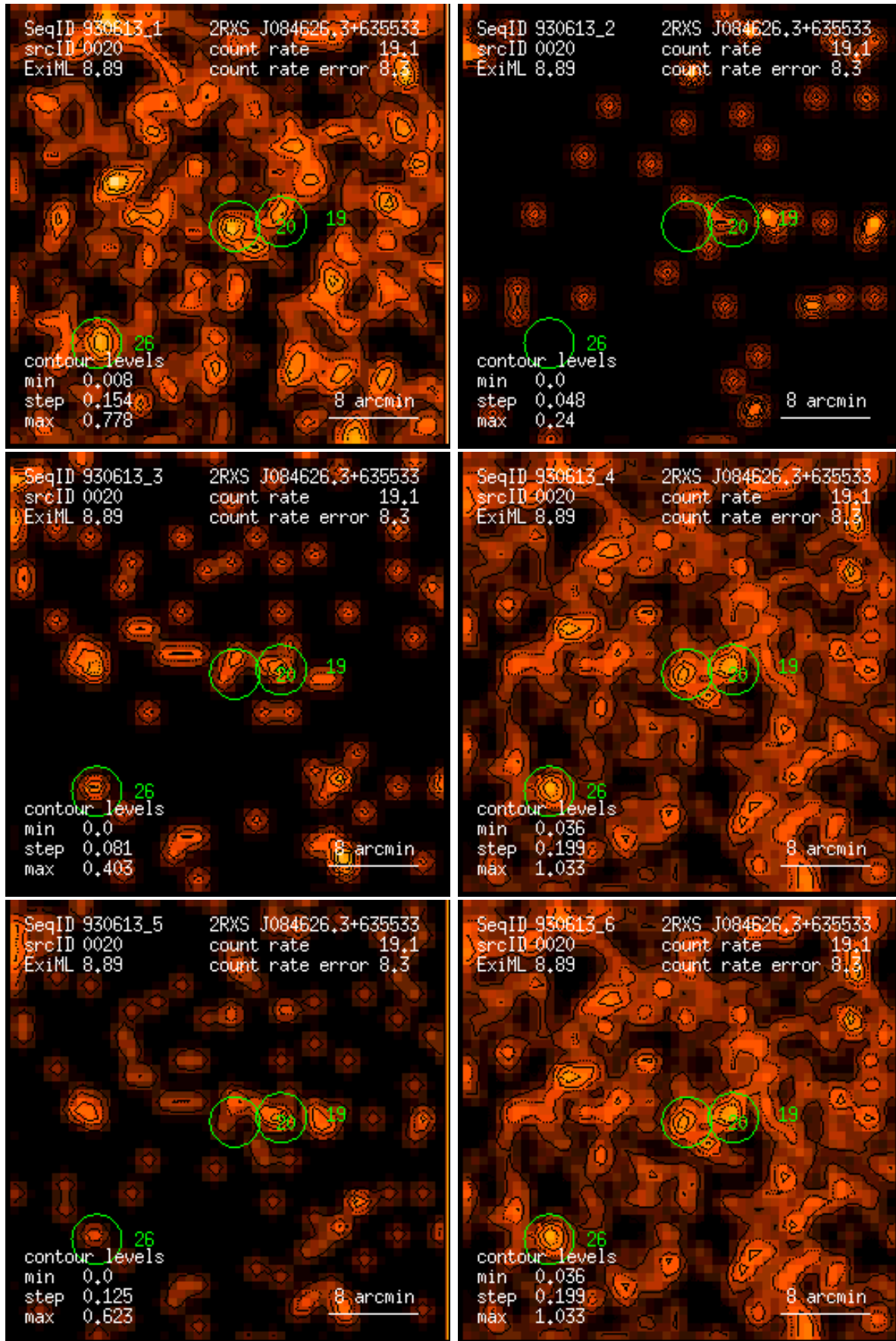
Figure 20: RASS 930613: detection 0020: band rate images, Gaussian filter: (1) PSPC channels 11 – 41, (2) 52 – 90, (3) 91 – 201, (4) 11 – 235, (5) 52 – 201, (6) 11 – 201. Broad band rates in counts/ks. Band rate contour levels in counts/ks/arcmin 2 .
