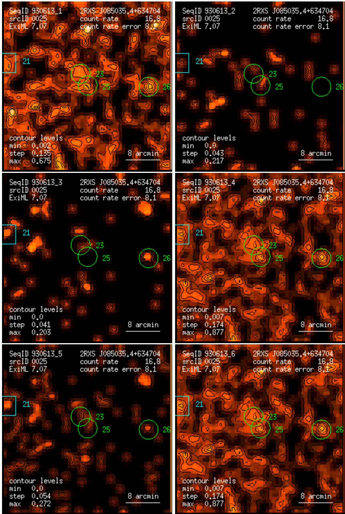
Figure 25: RASS 930613: detection 0025: band rate images, Gaussian filter: (1) PSPC channels 11 – 41, (2) 52 – 90, (3) 91 – 201, (4) 11 – 235, (5) 52 – 201, (6) 11 – 201. Broad band rates in counts/ks. Band rate contour levels in counts/ks/arcmin 2 .
