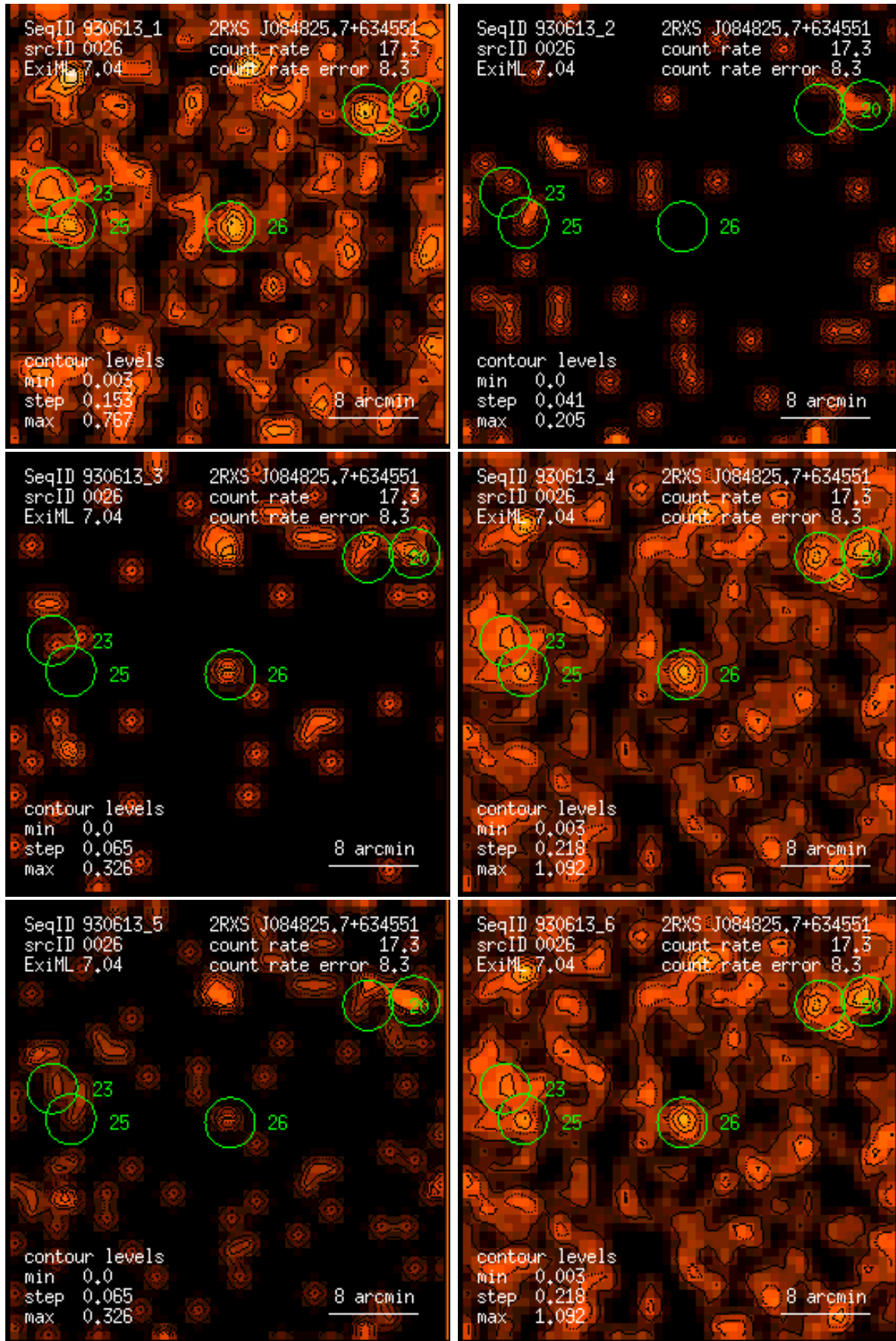
Figure 26: RASS 930613: detection 0026: band rate images, Gaussian filter: (1) PSPC channels 11 – 41, (2) 52 – 90, (3) 91 – 201, (4) 11 – 235, (5) 52 – 201, (6) 11 – 201. Broad band rates in counts/ks. Band rate contour levels in counts/ks/arcmin 2 .
