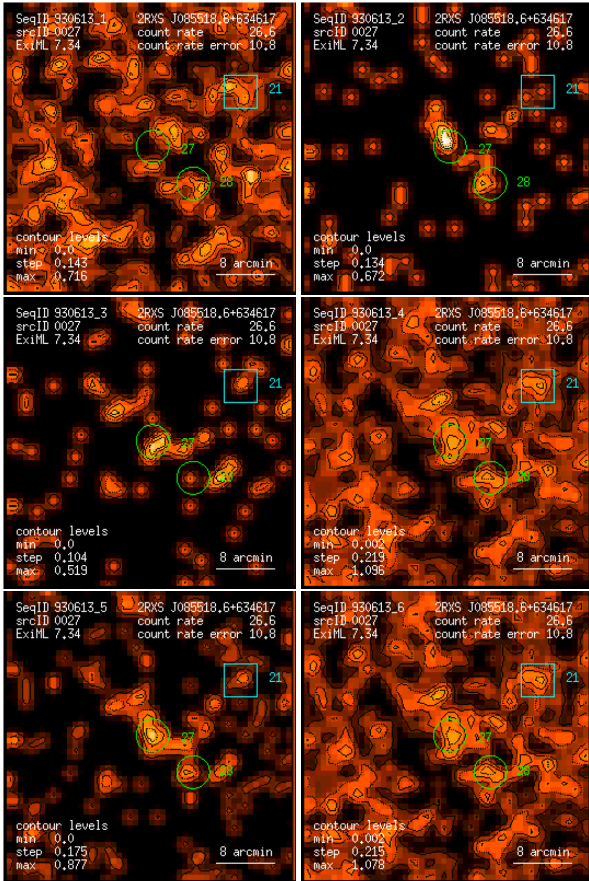
Figure 27: RASS 930613: detection 0027: band rate images, Gaussian filter: (1) PSPC channels 11 – 41, (2) 52 – 90, (3) 91 – 201, (4) 11 – 235, (5) 52 – 201, (6) 11 – 201. Broad band rates in counts/ks. Band rate contour levels in counts/ks/arcmin 2 .
