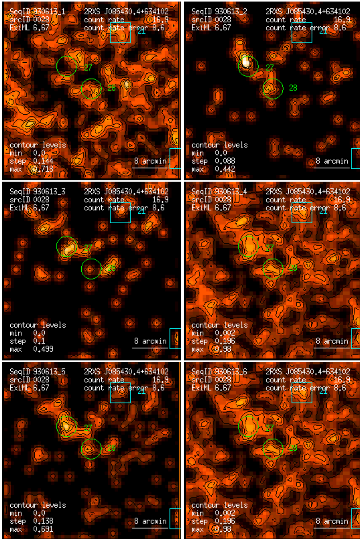
Figure 28: RASS 930613: detection 0028: band rate images, Gaussian filter: (1) PSPC channels 11 – 41, (2) 52 – 90, (3) 91 – 201, (4) 11 – 235, (5) 52 – 201, (6) 11 – 201. Broad band rates in counts/ks. Band rate contour levels in counts/ks/arcmin 2 .
