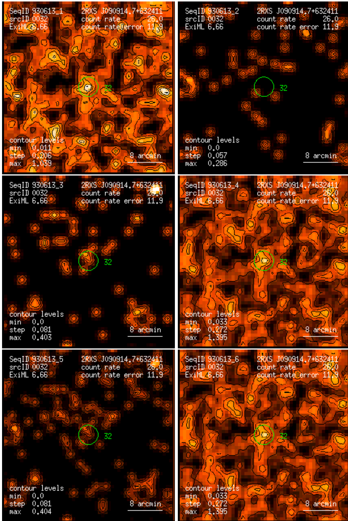
Figure 32: RASS 930613: detection 0032: band rate images, Gaussian filter: (1) PSPC channels 11 – 41, (2) 52 – 90, (3) 91 – 201, (4) 11 – 235, (5) 52 – 201, (6) 11 – 201. Broad band rates in counts/ks. Band rate contour levels in counts/ks/arcmin 2 .
