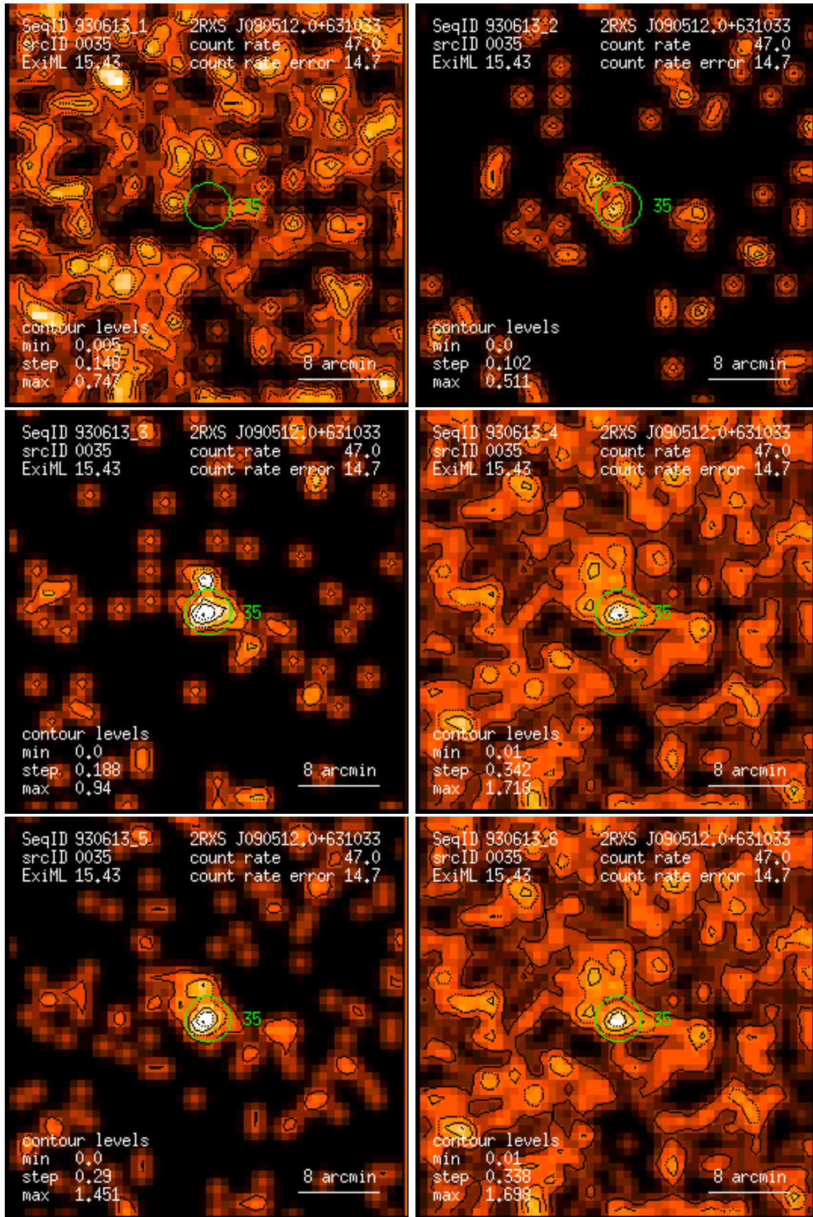
Figure 35: RASS 930613: detection 0035: band rate images, Gaussian filter: (1) PSPC channels 11 – 41, (2) 52 – 90, (3) 91 – 201, (4) 11 – 235, (5) 52 – 201, (6) 11 – 201. Broad band rates in counts/ks. Band rate contour levels in counts/ks/arcmin 2 .
