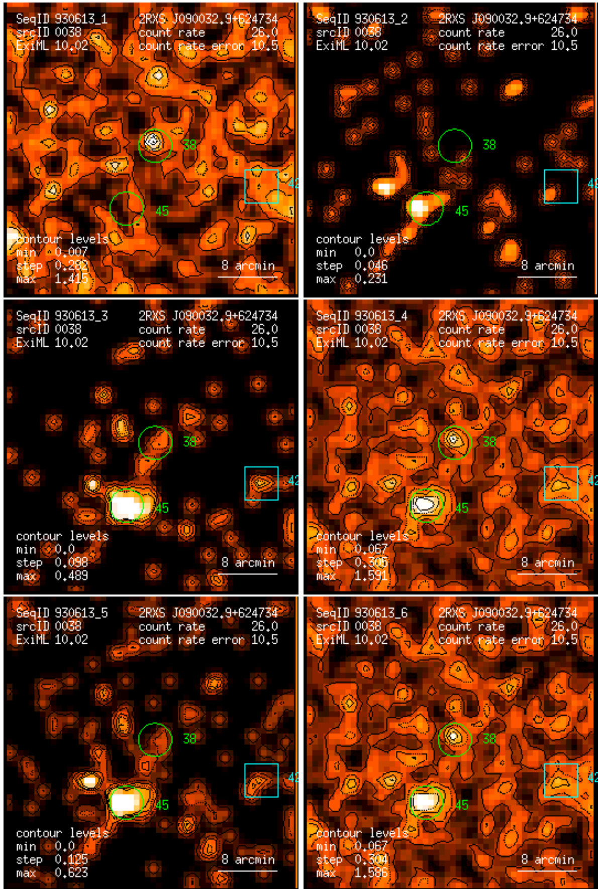
Figure 38: RASS 930613: detection 0038: band rate images, Gaussian filter: (1) PSPC channels 11 – 41, (2) 52 – 90, (3) 91 – 201, (4) 11 – 235, (5) 52 – 201, (6) 11 – 201. Broad band rates in counts/ks. Band rate contour levels in counts/ks/arcmin 2 .
