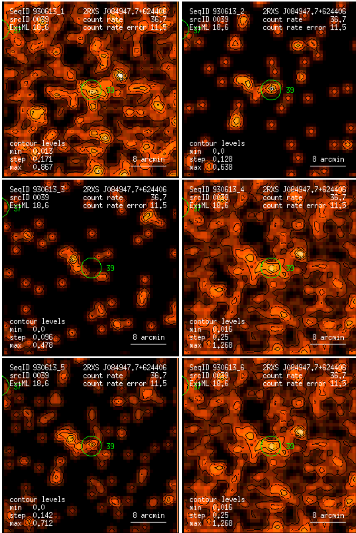
Figure 39: RASS 930613: detection 0039: band rate images, Gaussian filter: (1) PSPC channels 11 – 41, (2) 52 – 90, (3) 91 – 201, (4) 11 – 235, (5) 52 – 201, (6) 11 – 201. Broad band rates in counts/ks. Band rate contour levels in counts/ks/arcmin 2 .
