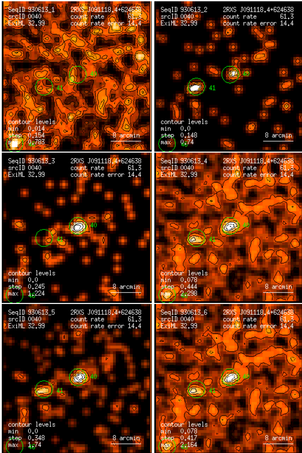
Figure 40: RASS 930613: detection 0040: band rate images, Gaussian filter: (1) PSPC channels 11 – 41, (2) 52 – 90, (3) 91 – 201, (4) 11 – 235, (5) 52 – 201, (6) 11 – 201. Broad band rates in counts/ks. Band rate contour levels in counts/ks/arcmin 2 .
