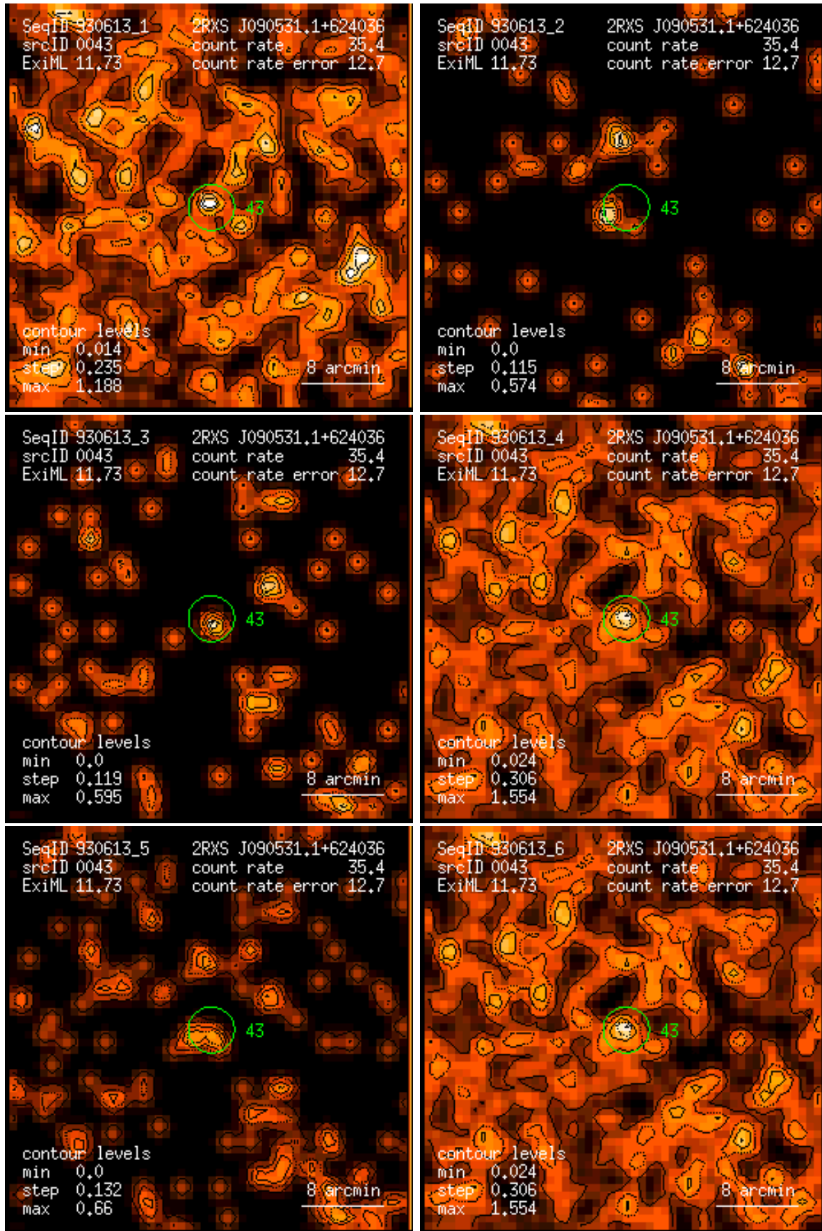
Figure 43: RASS 930613: detection 0043: band rate images, Gaussian filter: (1) PSPC channels 11 – 41, (2) 52 – 90, (3) 91 – 201, (4) 11 – 235, (5) 52 – 201, (6) 11 – 201. Broad band rates in counts/ks. Band rate contour levels in counts/ks/arcmin 2 .
