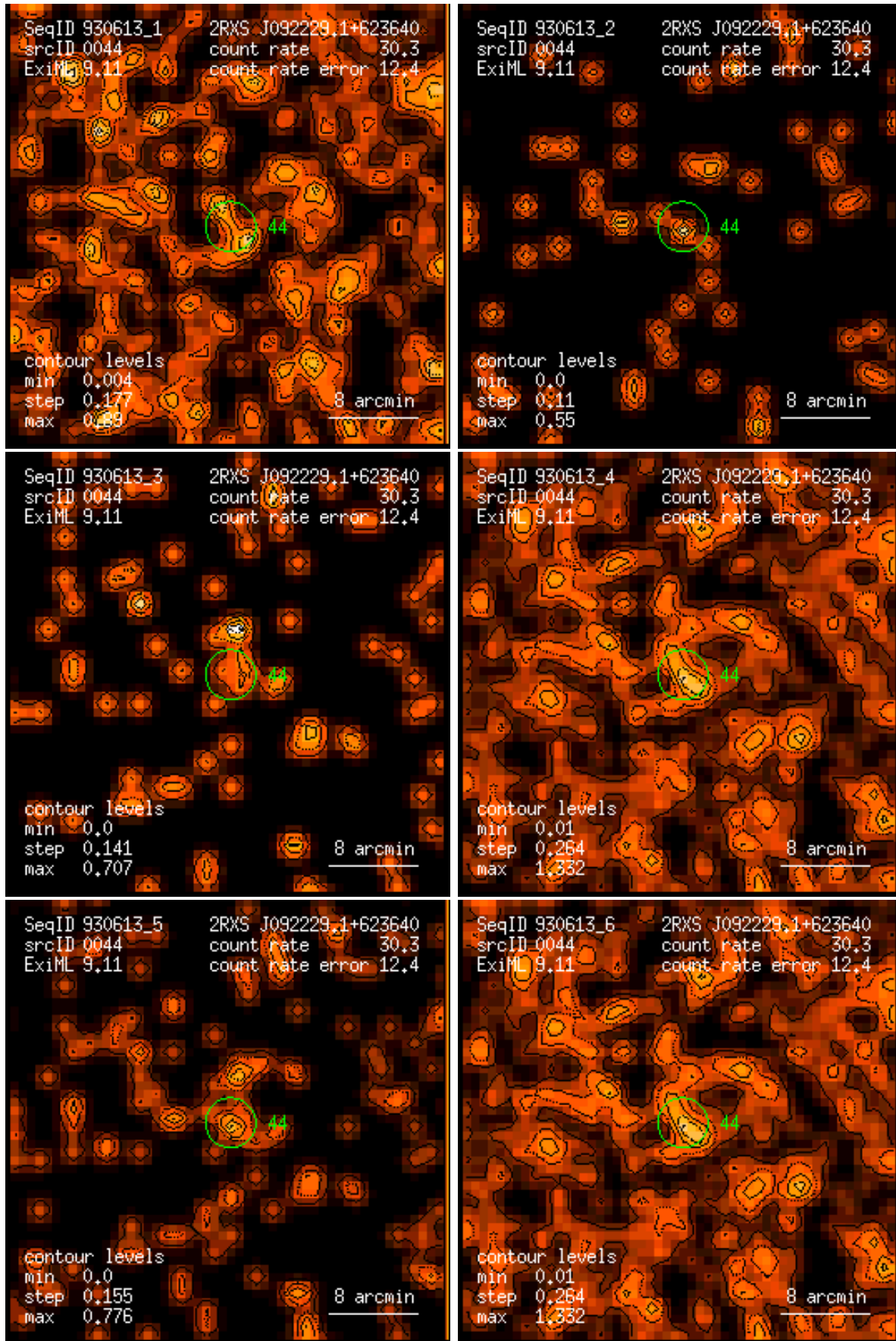
Figure 44: RASS 930613: detection 0044: band rate images, Gaussian filter: (1) PSPC channels 11 – 41, (2) 52 – 90, (3) 91 – 201, (4) 11 – 235, (5) 52 – 201, (6) 11 – 201. Broad band rates in counts/ks. Band rate contour levels in counts/ks/arcmin 2 .
