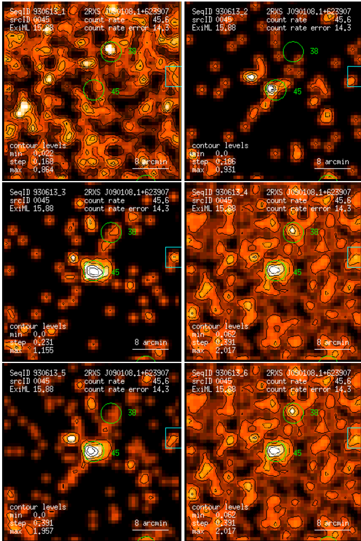
Figure 45: RASS 930613: detection 0045: band rate images, Gaussian filter: (1) PSPC channels 11 – 41, (2) 52 – 90, (3) 91 – 201, (4) 11 – 235, (5) 52 – 201, (6) 11 – 201. Broad band rates in counts/ks. Band rate contour levels in counts/ks/arcmin 2 .
