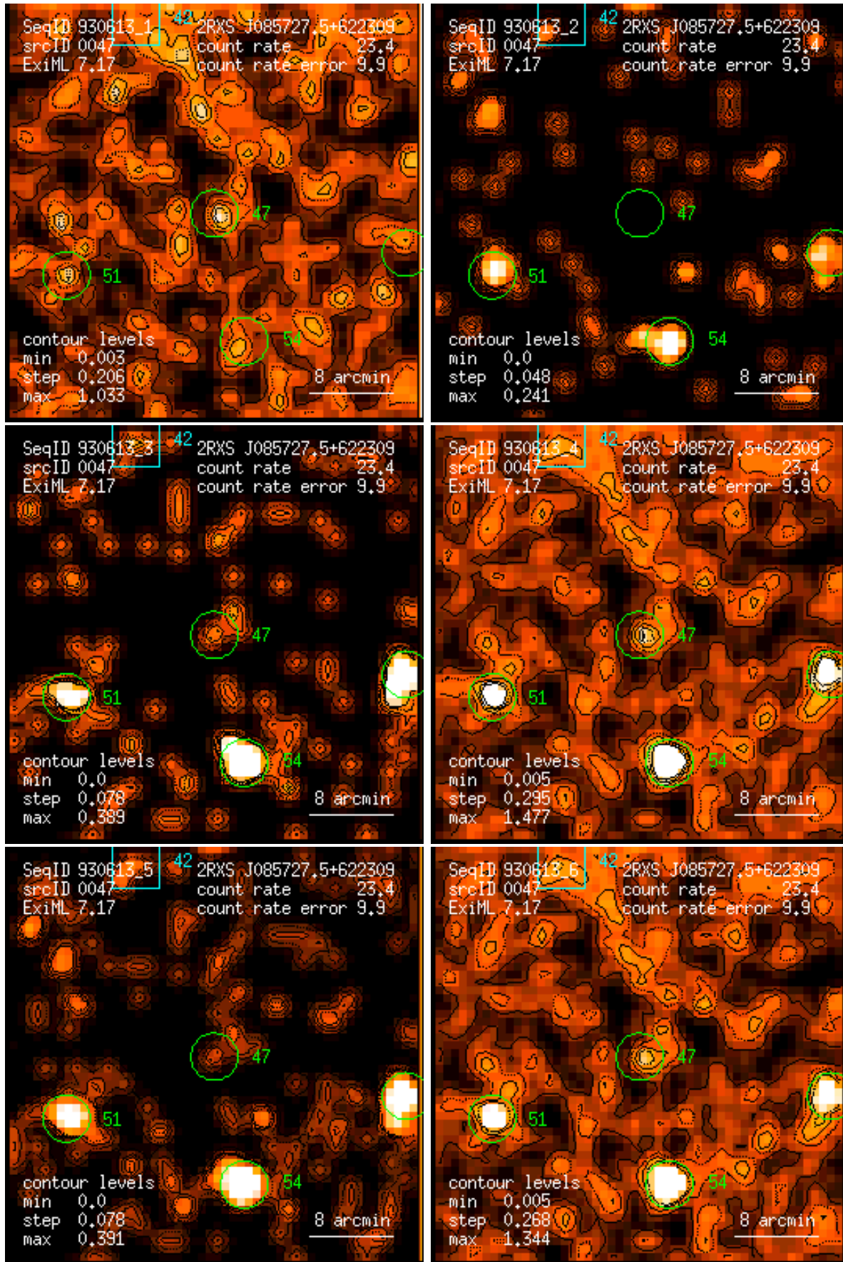
Figure 47: RASS 930613: detection 0047: band rate images, Gaussian filter: (1) PSPC channels 11 – 41, (2) 52 – 90, (3) 91 – 201, (4) 11 – 235, (5) 52 – 201, (6) 11 – 201. Broad band rates in counts/ks. Band rate contour levels in counts/ks/arcmin 2 .
