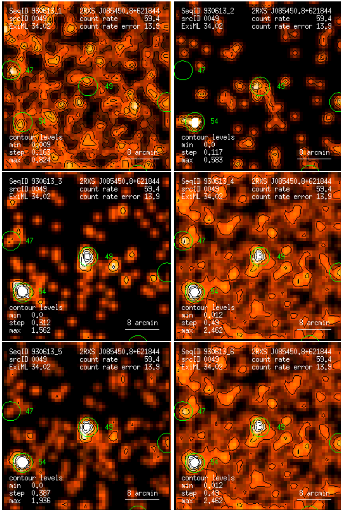
Figure 49: RASS 930613: detection 0049: band rate images, Gaussian filter: (1) PSPC channels 11 – 41, (2) 52 – 90, (3) 91 – 201, (4) 11 – 235, (5) 52 – 201, (6) 11 – 201. Broad band rates in counts/ks. Band rate contour levels in counts/ks/arcmin 2 .
