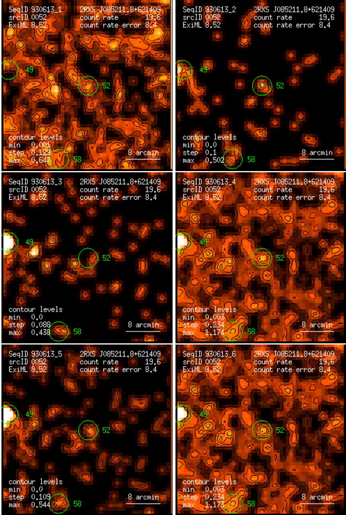
Figure 52: RASS 930613: detection 0052: band rate images, Gaussian filter: (1) PSPC channels 11 – 41, (2) 52 – 90, (3) 91 – 201, (4) 11 – 235, (5) 52 – 201, (6) 11 – 201. Broad band rates in counts/ks. Band rate contour levels in counts/ks/arcmin 2 .
