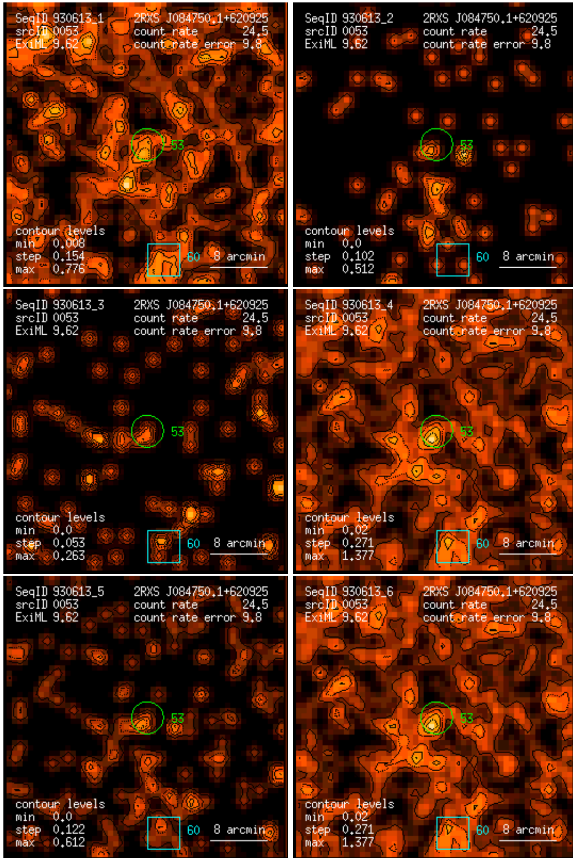
Figure 53: RASS 930613: detection 0053: band rate images, Gaussian filter: (1) PSPC channels 11 – 41, (2) 52 – 90, (3) 91 – 201, (4) 11 – 235, (5) 52 – 201, (6) 11 – 201. Broad band rates in counts/ks. Band rate contour levels in counts/ks/arcmin 2 .
