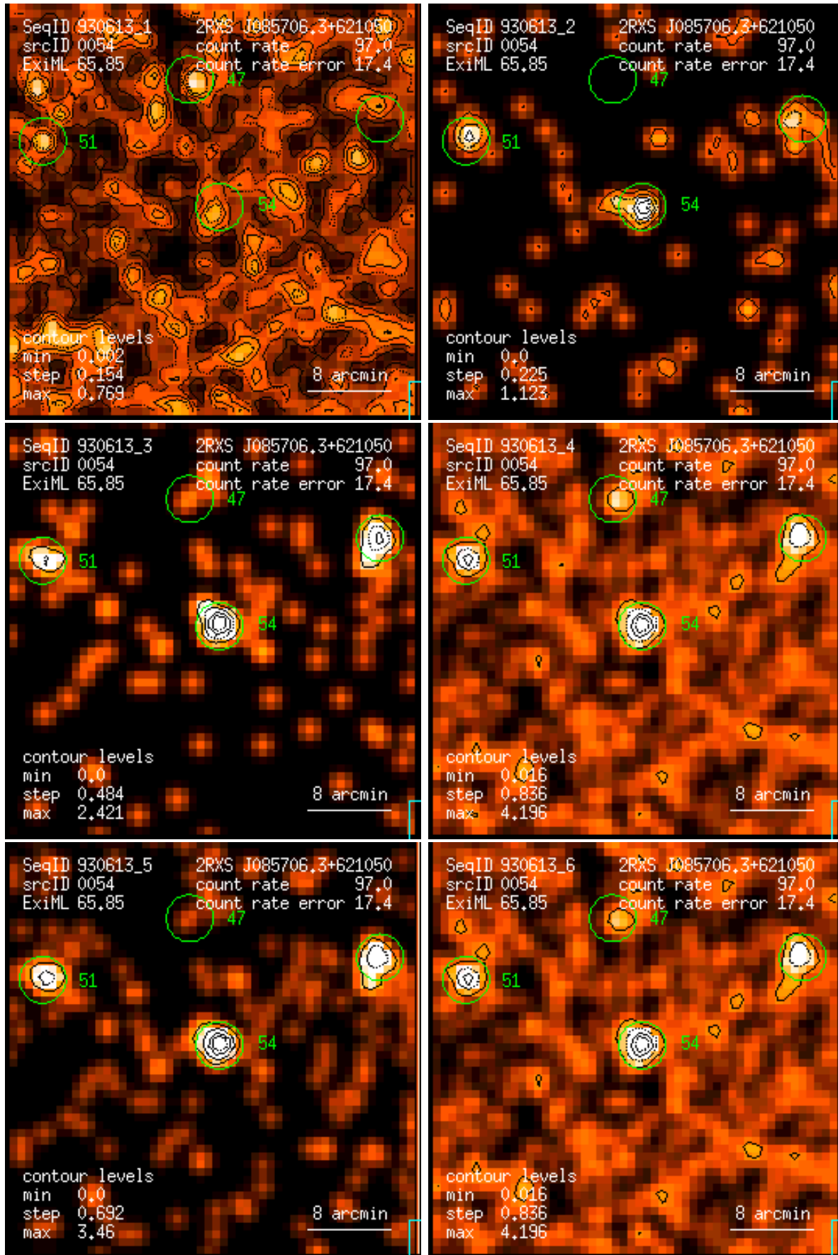
Figure 54: RASS 930613: detection 0054: band rate images, Gaussian filter: (1) PSPC channels 11 – 41, (2) 52 – 90, (3) 91 – 201, (4) 11 – 235, (5) 52 – 201, (6) 11 – 201. Broad band rates in counts/ks. Band rate contour levels in counts/ks/arcmin 2 .
