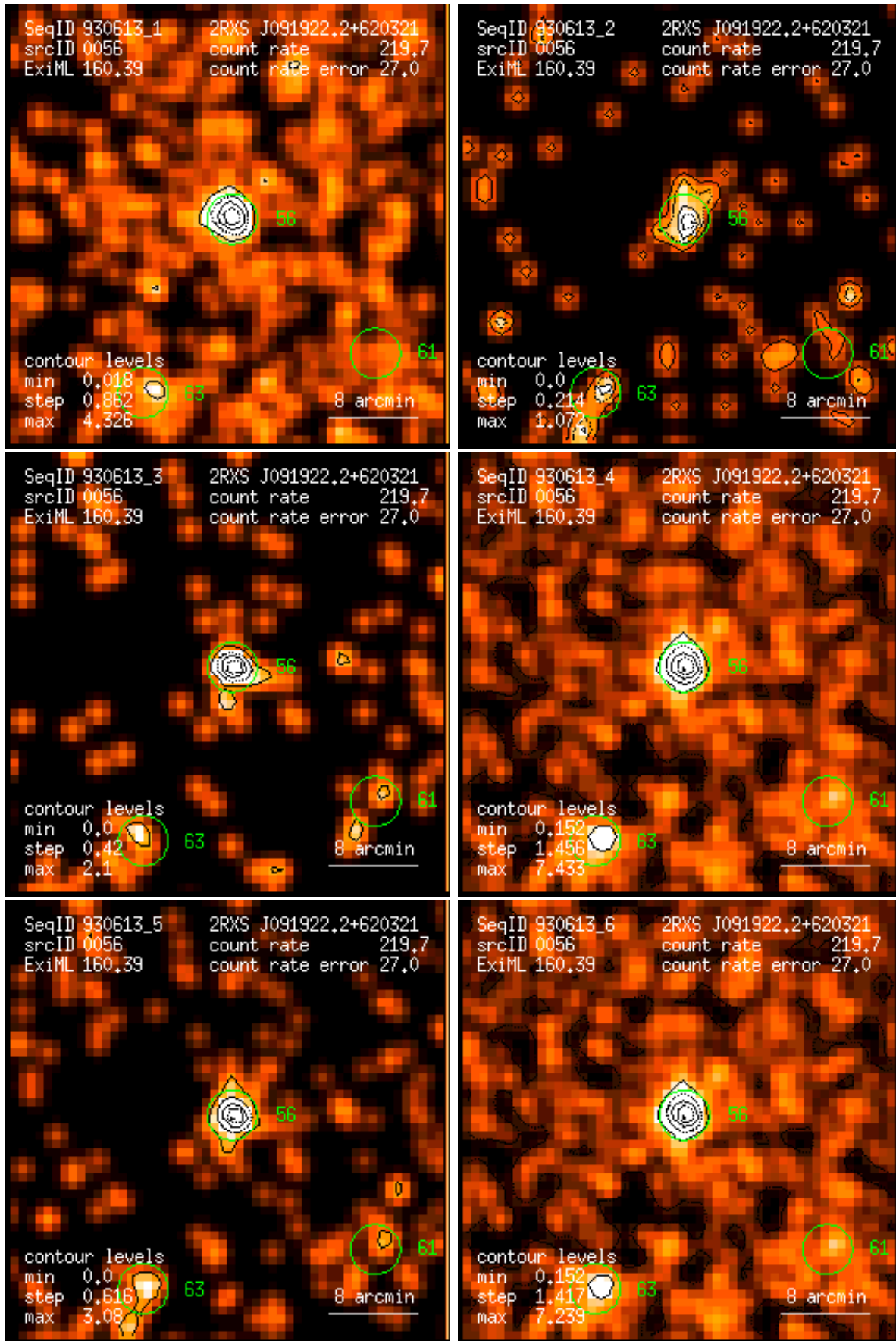
Figure 56: RASS 930613: detection 0056: band rate images, Gaussian filter: (1) PSPC channels 11 – 41, (2) 52 – 90, (3) 91 – 201, (4) 11 – 235, (5) 52 – 201, (6) 11 – 201. Broad band rates in counts/ks. Band rate contour levels in counts/ks/arcmin 2 .
