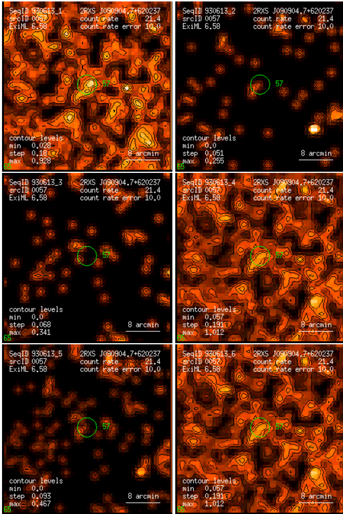
Figure 57: RASS 930613: detection 0057: band rate images, Gaussian filter: (1) PSPC channels 11 – 41, (2) 52 – 90, (3) 91 – 201, (4) 11 – 235, (5) 52 – 201, (6) 11 – 201. Broad band rates in counts/ks. Band rate contour levels in counts/ks/arcmin 2 .
