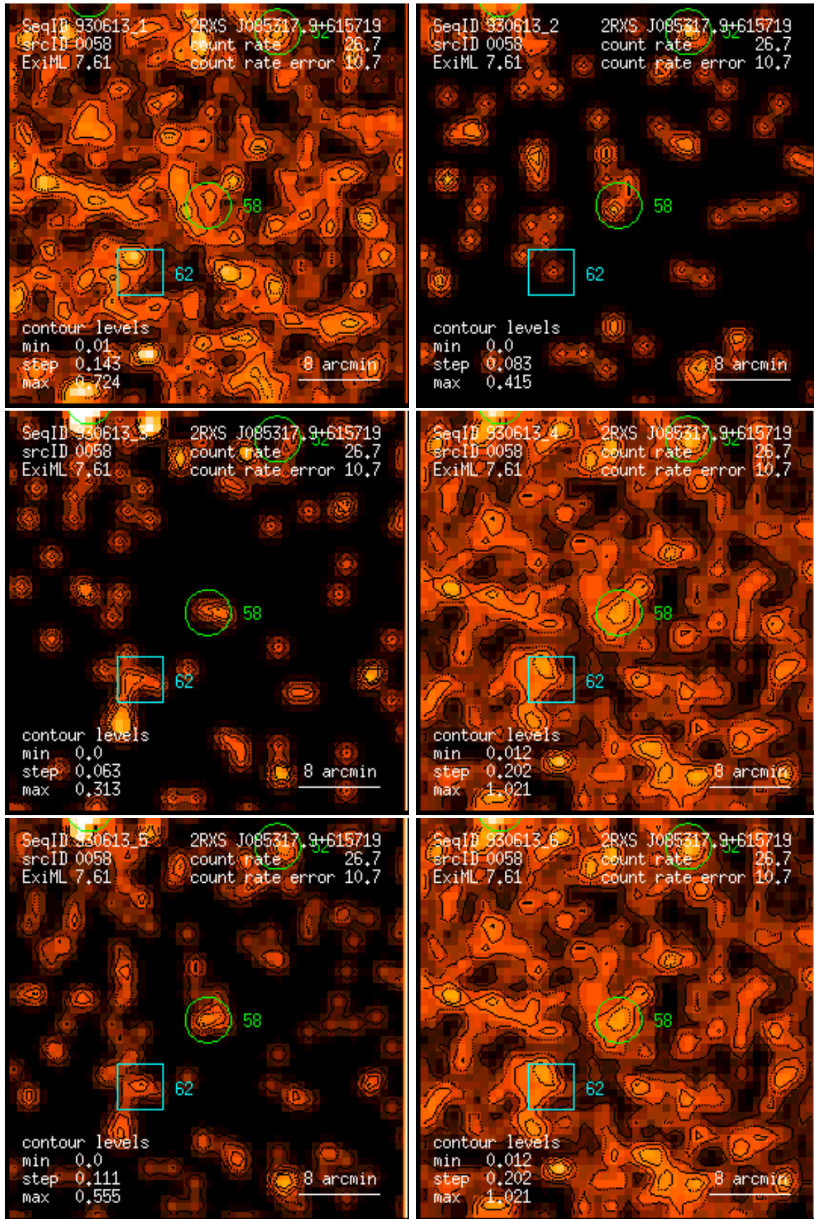
Figure 58: RASS 930613: detection 0058: band rate images, Gaussian filter: (1) PSPC channels 11 – 41, (2) 52 – 90, (3) 91 – 201, (4) 11 – 235, (5) 52 – 201, (6) 11 – 201. Broad band rates in counts/ks. Band rate contour levels in counts/ks/arcmin 2 .
