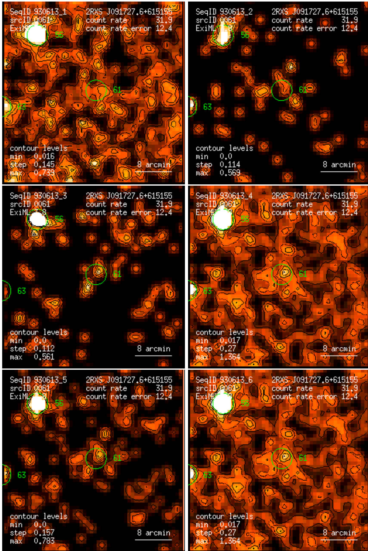
Figure 61: RASS 930613: detection 0061: band rate images, Gaussian filter: (1) PSPC channels 11 – 41, (2) 52 – 90, (3) 91 – 201, (4) 11 – 235, (5) 52 – 201, (6) 11 – 201. Broad band rates in counts/ks. Band rate contour levels in counts/ks/arcmin 2 .
