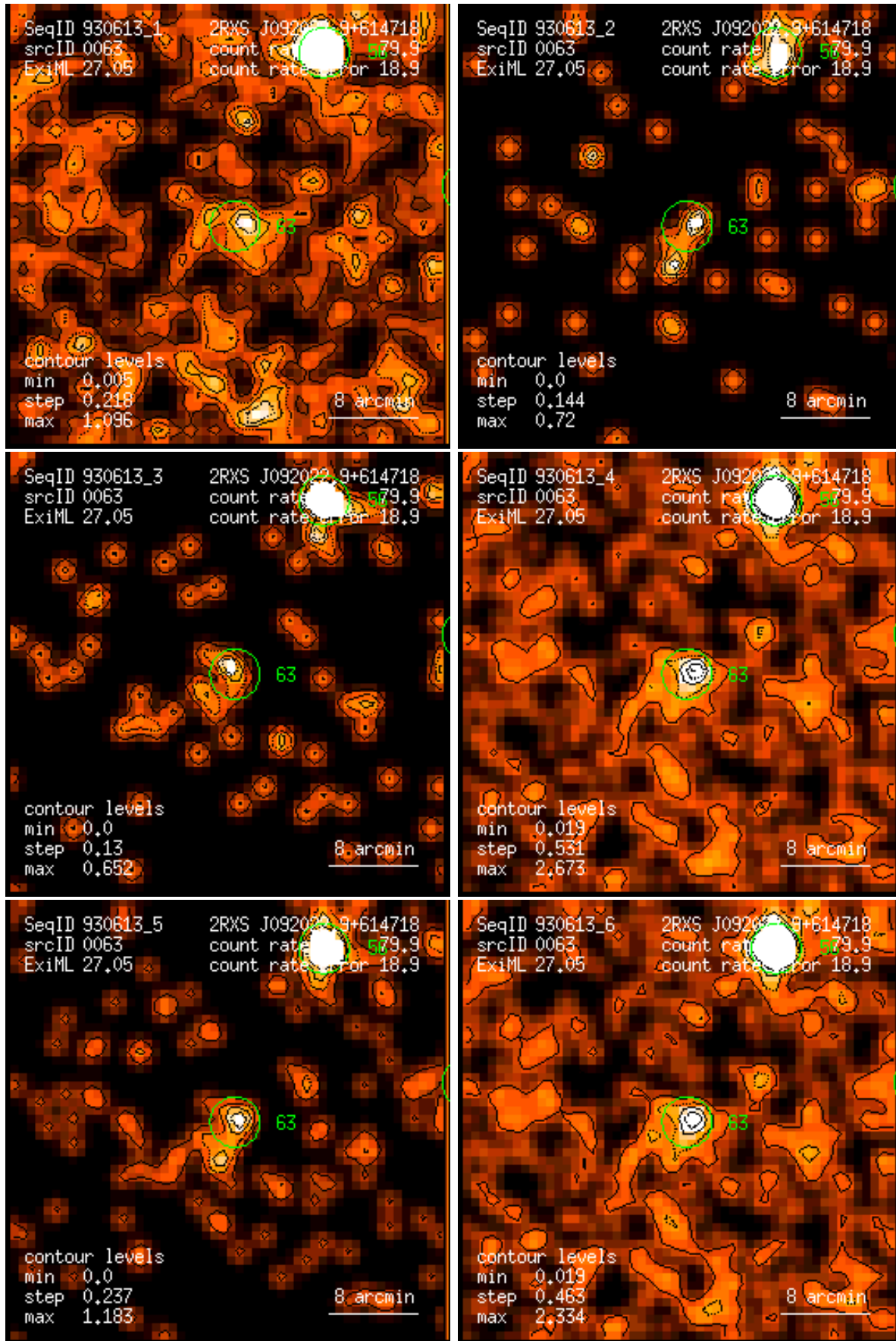
Figure 63: RASS 930613: detection 0063: band rate images, Gaussian filter: (1) PSPC channels 11 – 41, (2) 52 – 90, (3) 91 – 201, (4) 11 – 235, (5) 52 – 201, (6) 11 – 201. Broad band rates in counts/ks. Band rate contour levels in counts/ks/arcmin 2 .
