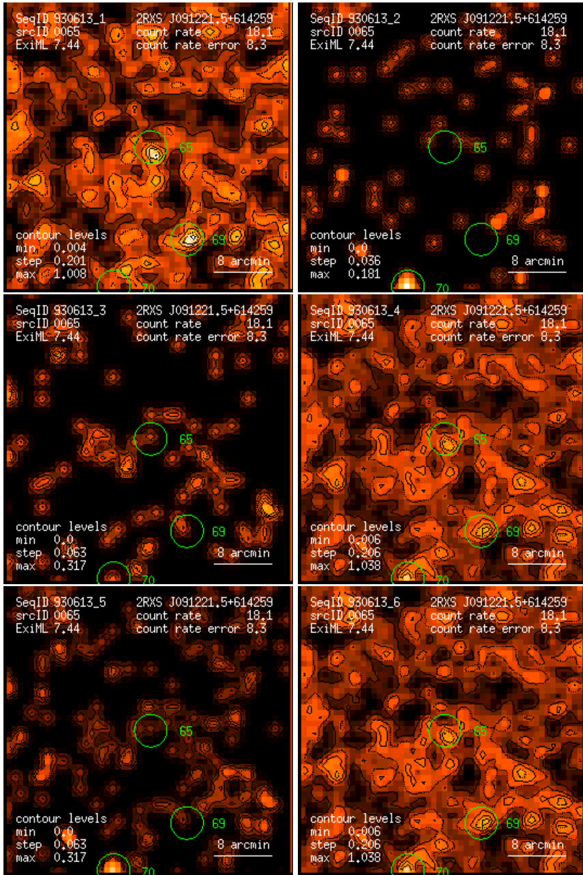
Figure 65: RASS 930613: detection 0065: band rate images, Gaussian filter: (1) PSPC channels 11 – 41, (2) 52 – 90, (3) 91 – 201, (4) 11 – 235, (5) 52 – 201, (6) 11 – 201. Broad band rates in counts/ks. Band rate contour levels in counts/ks/arcmin 2 .
