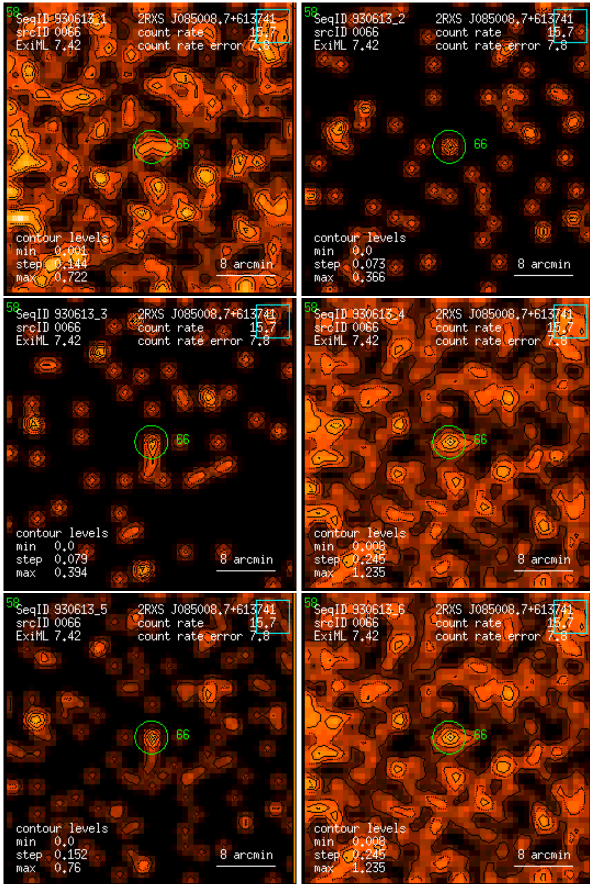
Figure 66: RASS 930613: detection 0066: band rate images, Gaussian filter: (1) PSPC channels 11 – 41, (2) 52 – 90, (3) 91 – 201, (4) 11 – 235, (5) 52 – 201, (6) 11 – 201. Broad band rates in counts/ks. Band rate contour levels in counts/ks/arcmin 2 .
