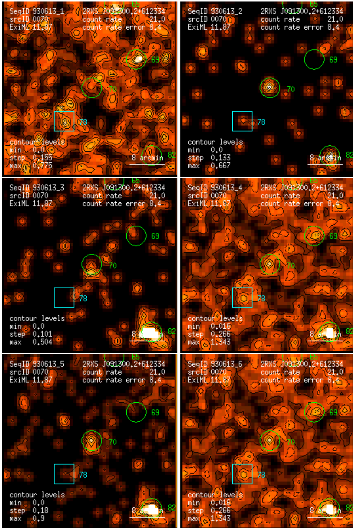
Figure 70: RASS 930613: detection 0070: band rate images, Gaussian filter: (1) PSPC channels 11 – 41, (2) 52 – 90, (3) 91 – 201, (4) 11 – 235, (5) 52 – 201, (6) 11 – 201. Broad band rates in counts/ks. Band rate contour levels in counts/ks/arcmin 2 .
