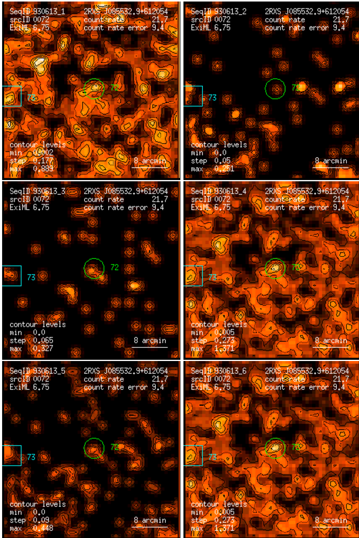
Figure 72: RASS 930613: detection 0072: band rate images, Gaussian filter: (1) PSPC channels 11 – 41, (2) 52 – 90, (3) 91 – 201, (4) 11 – 235, (5) 52 – 201, (6) 11 – 201. Broad band rates in counts/ks. Band rate contour levels in counts/ks/arcmin 2 .
