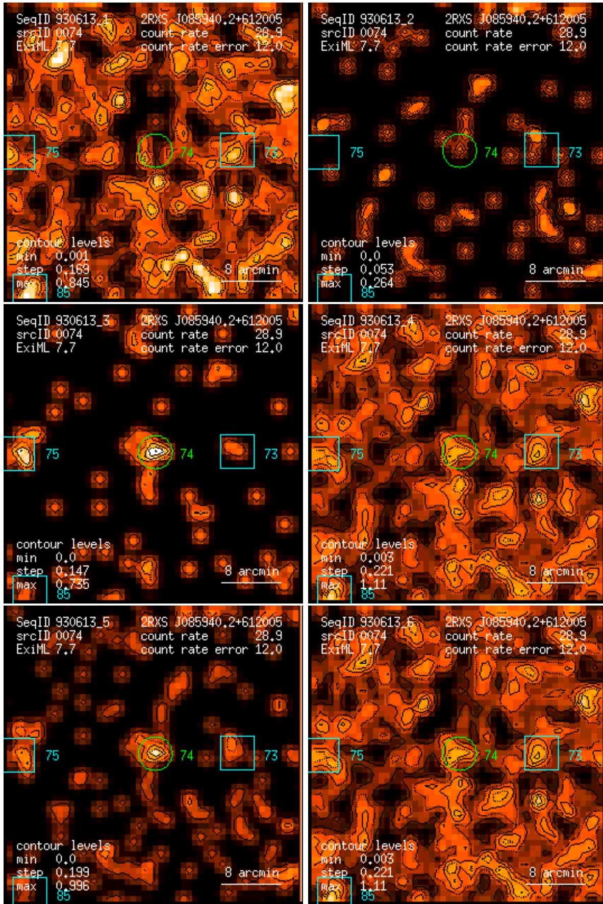
Figure 74: RASS 930613: detection 0074: band rate images, Gaussian filter: (1) PSPC channels 11 – 41, (2) 52 – 90, (3) 91 – 201, (4) 11 – 235, (5) 52 – 201, (6) 11 – 201. Broad band rates in counts/ks. Band rate contour levels in counts/ks/arcmin 2 .
