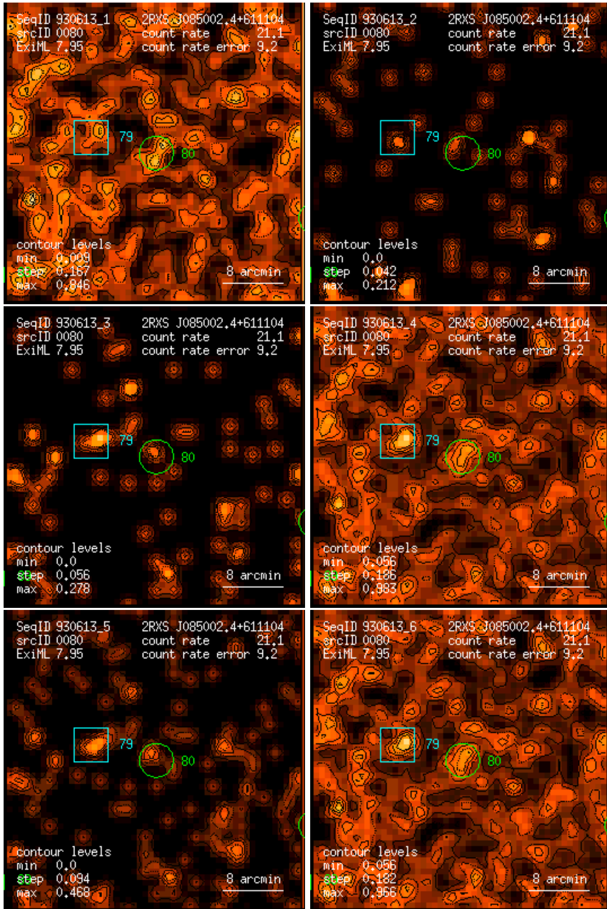
Figure 80: RASS 930613: detection 0080: band rate images, Gaussian filter: (1) PSPC channels 11 – 41, (2) 52 – 90, (3) 91 – 201, (4) 11 – 235, (5) 52 – 201, (6) 11 – 201. Broad band rates in counts/ks. Band rate contour levels in counts/ks/arcmin 2 .
