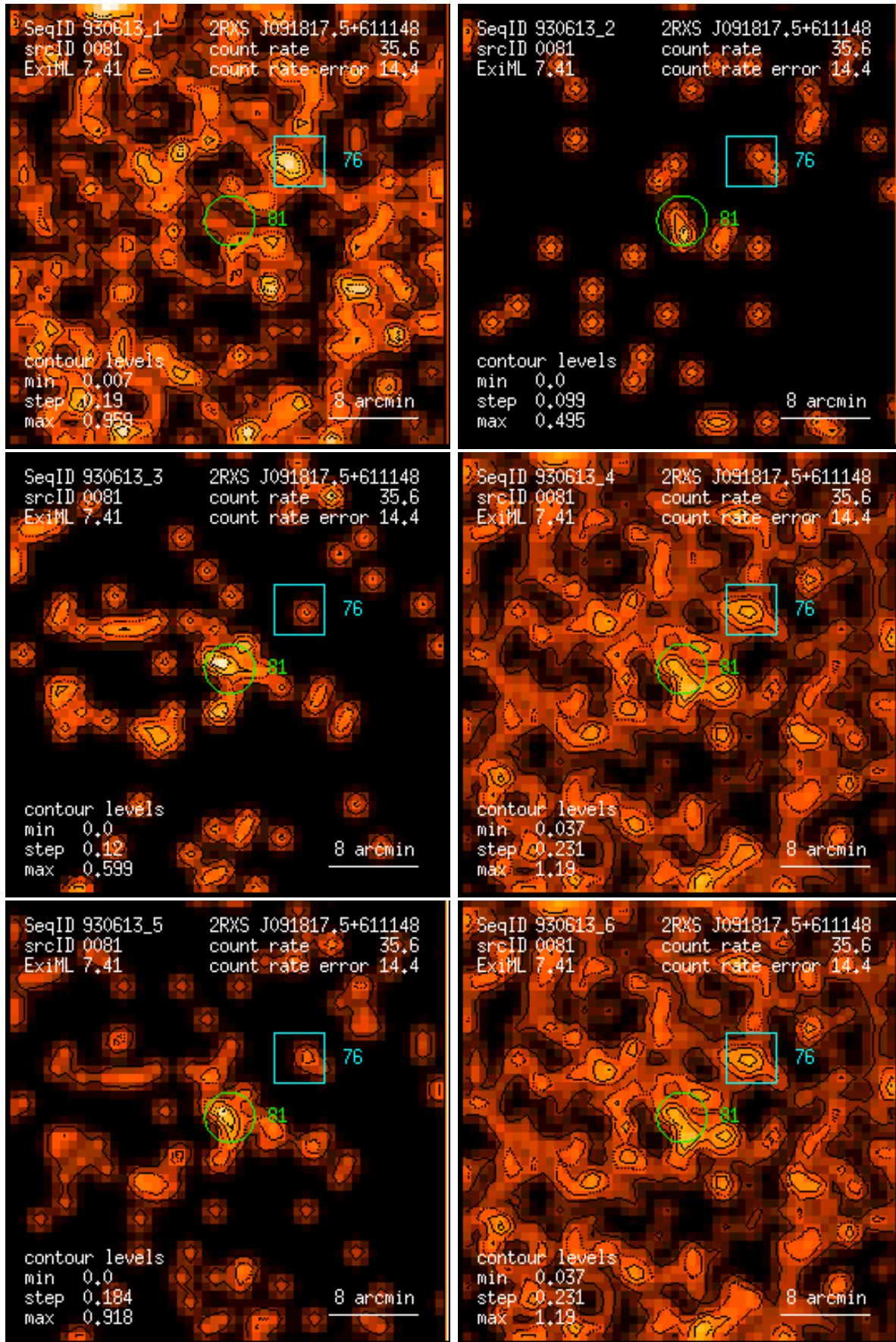
Figure 81: RASS 930613: detection 0081: band rate images, Gaussian filter: (1) PSPC channels 11 – 41, (2) 52 – 90, (3) 91 – 201, (4) 11 – 235, (5) 52 – 201, (6) 11 – 201. Broad band rates in counts/ks. Band rate contour levels in counts/ks/arcmin 2 .
