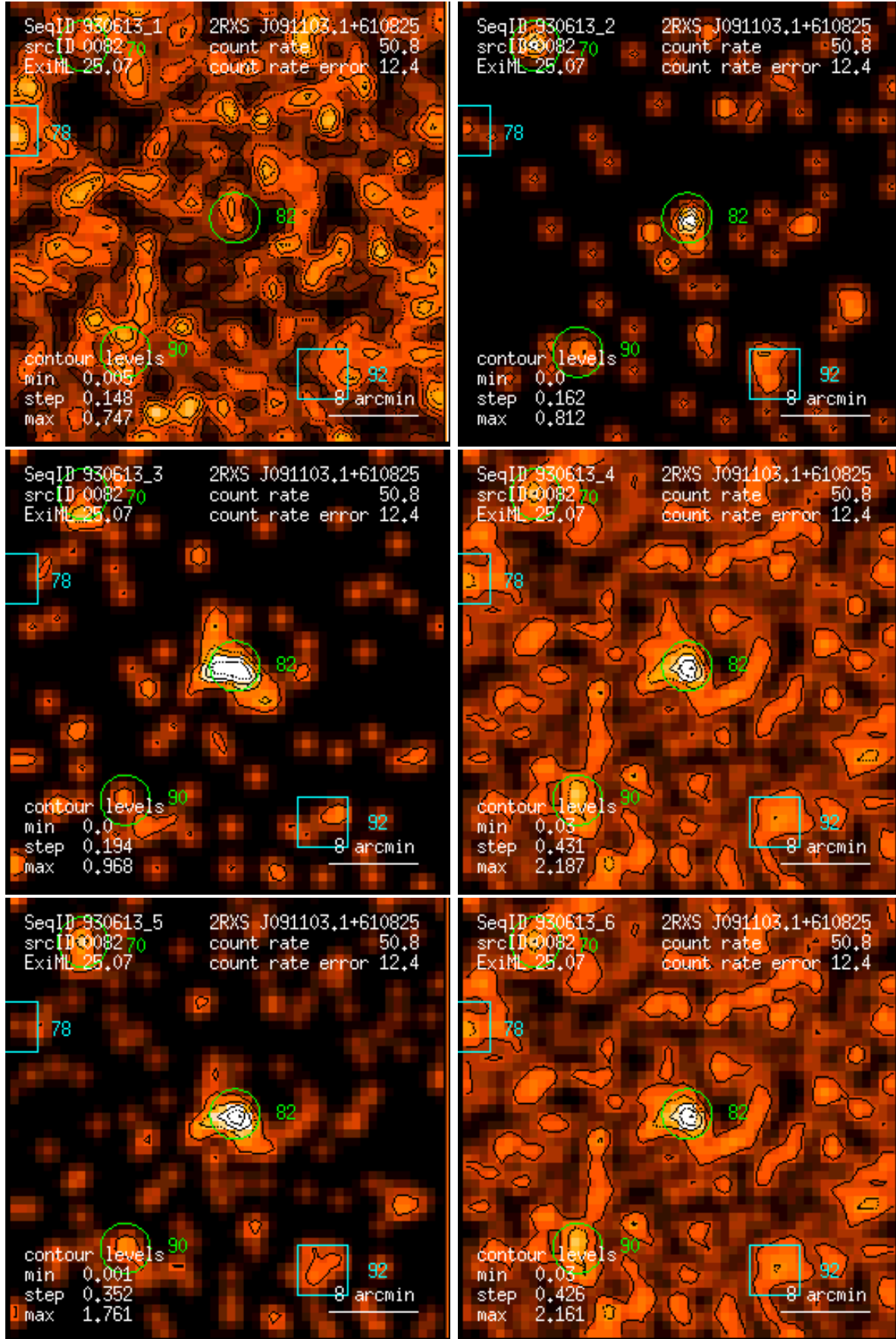
Figure 82: RASS 930613: detection 0082: band rate images, Gaussian filter: (1) PSPC channels 11 – 41, (2) 52 – 90, (3) 91 – 201, (4) 11 – 235, (5) 52 – 201, (6) 11 – 201. Broad band rates in counts/ks. Band rate contour levels in counts/ks/arcmin 2 .
