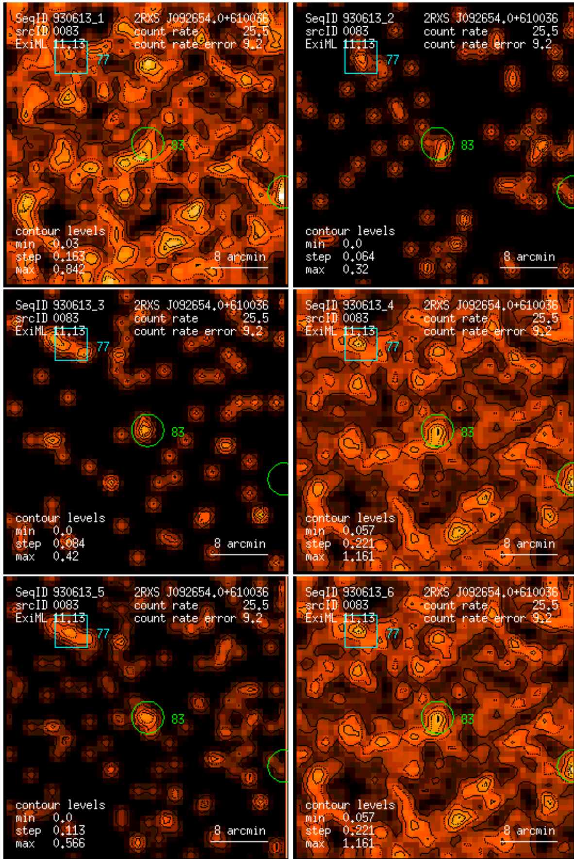
Figure 83: RASS 930613: detection 0083: band rate images, Gaussian filter: (1) PSPC channels 11 – 41, (2) 52 – 90, (3) 91 – 201, (4) 11 – 235, (5) 52 – 201, (6) 11 – 201. Broad band rates in counts/ks. Band rate contour levels in counts/ks/arcmin 2 .
