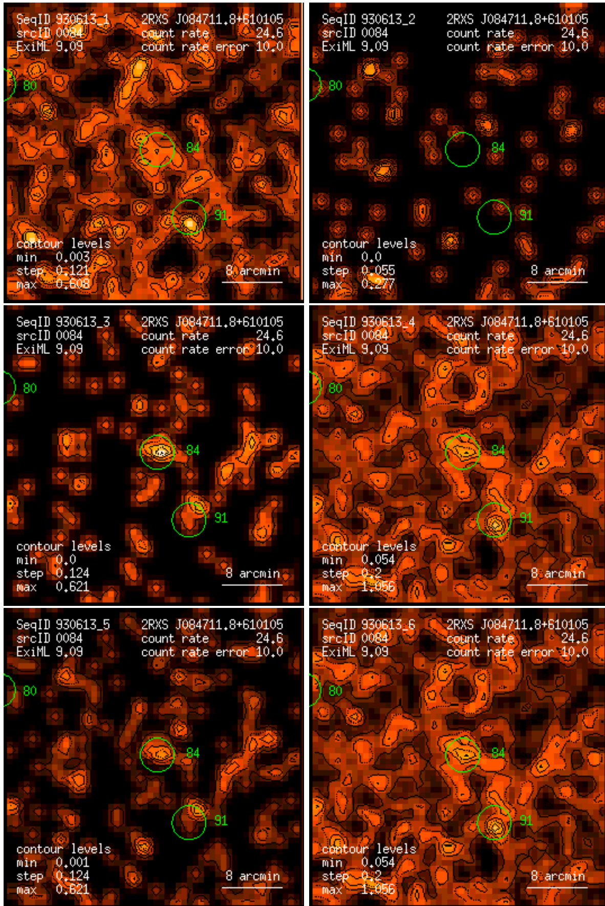
Figure 84: RASS 930613: detection 0084: band rate images, Gaussian filter: (1) PSPC channels 11 – 41, (2) 52 – 90, (3) 91 – 201, (4) 11 – 235, (5) 52 – 201, (6) 11 – 201. Broad band rates in counts/ks. Band rate contour levels in counts/ks/arcmin 2 .
