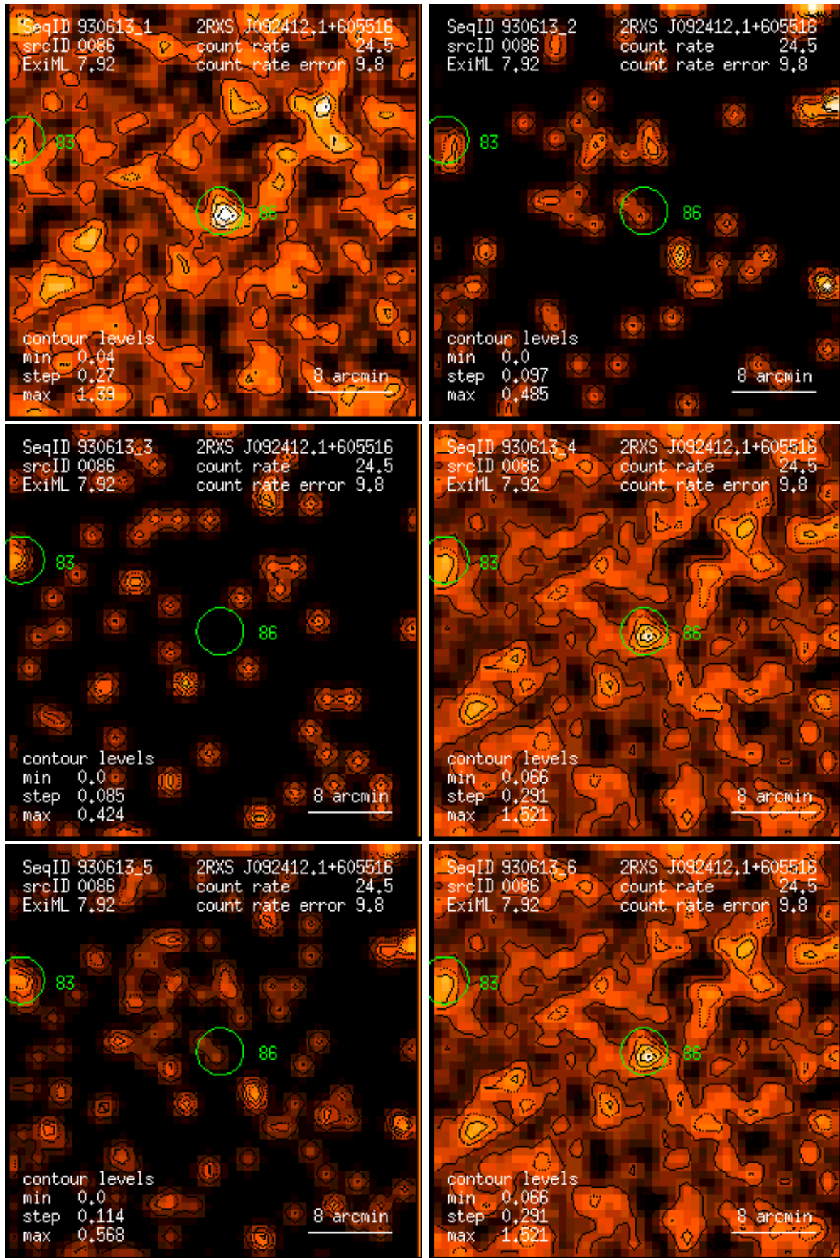
Figure 86: RASS 930613: detection 0086: band rate images, Gaussian filter: (1) PSPC channels 11 – 41, (2) 52 – 90, (3) 91 – 201, (4) 11 – 235, (5) 52 – 201, (6) 11 – 201. Broad band rates in counts/ks. Band rate contour levels in counts/ks/arcmin 2 .
