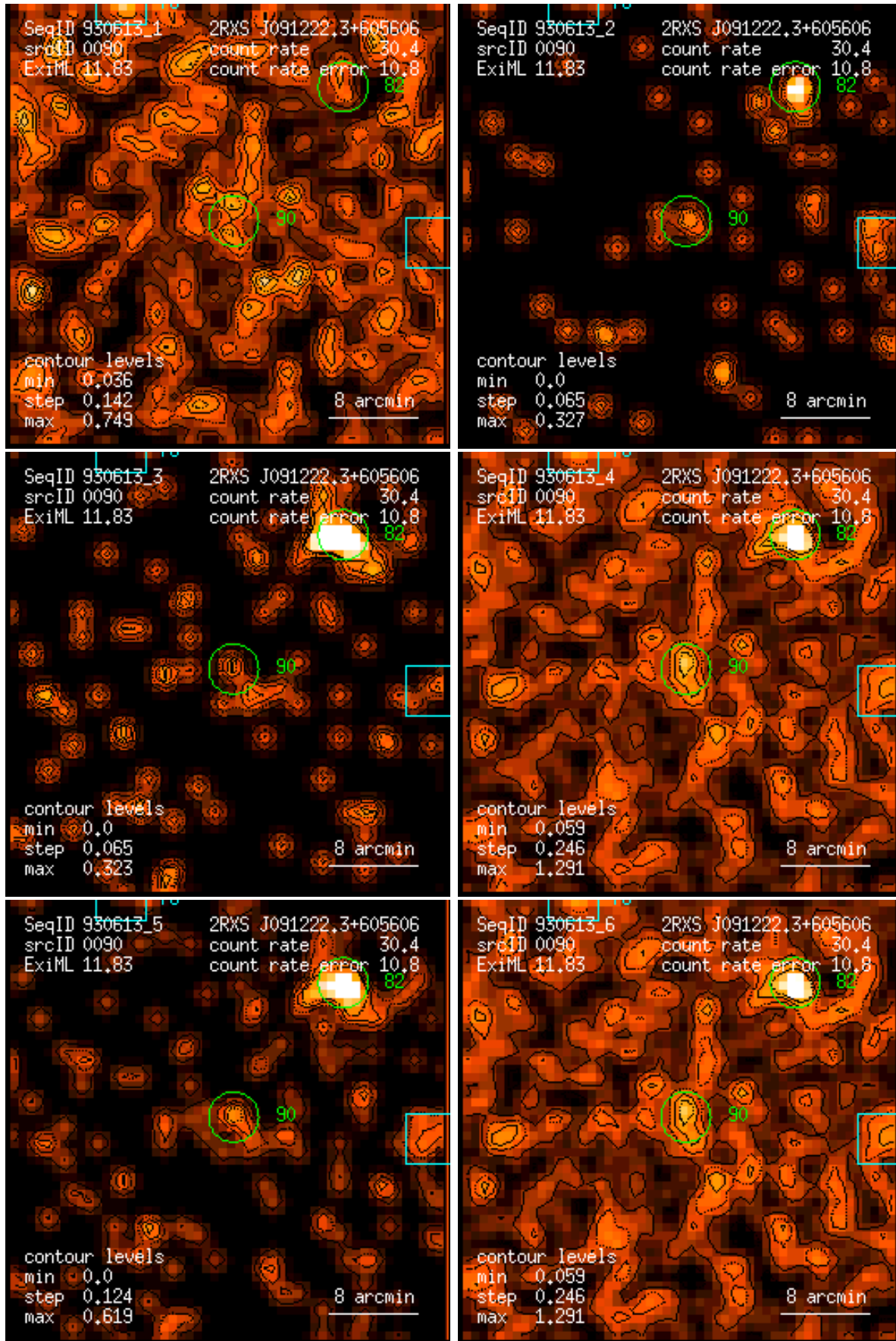
Figure 90: RASS 930613: detection 0090: band rate images, Gaussian filter: (1) PSPC channels 11 – 41, (2) 52 – 90, (3) 91 – 201, (4) 11 – 235, (5) 52 – 201, (6) 11 – 201. Broad band rates in counts/ks. Band rate contour levels in counts/ks/arcmin 2 .
