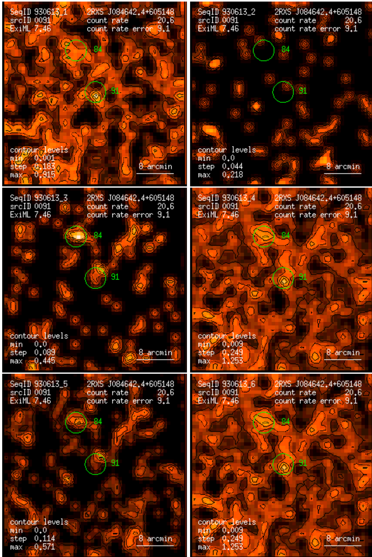
Figure 91: RASS 930613: detection 0091: band rate images, Gaussian filter: (1) PSPC channels 11 – 41, (2) 52 – 90, (3) 91 – 201, (4) 11 – 235, (5) 52 – 201, (6) 11 – 201. Broad band rates in counts/ks. Band rate contour levels in counts/ks/arcmin 2 .
