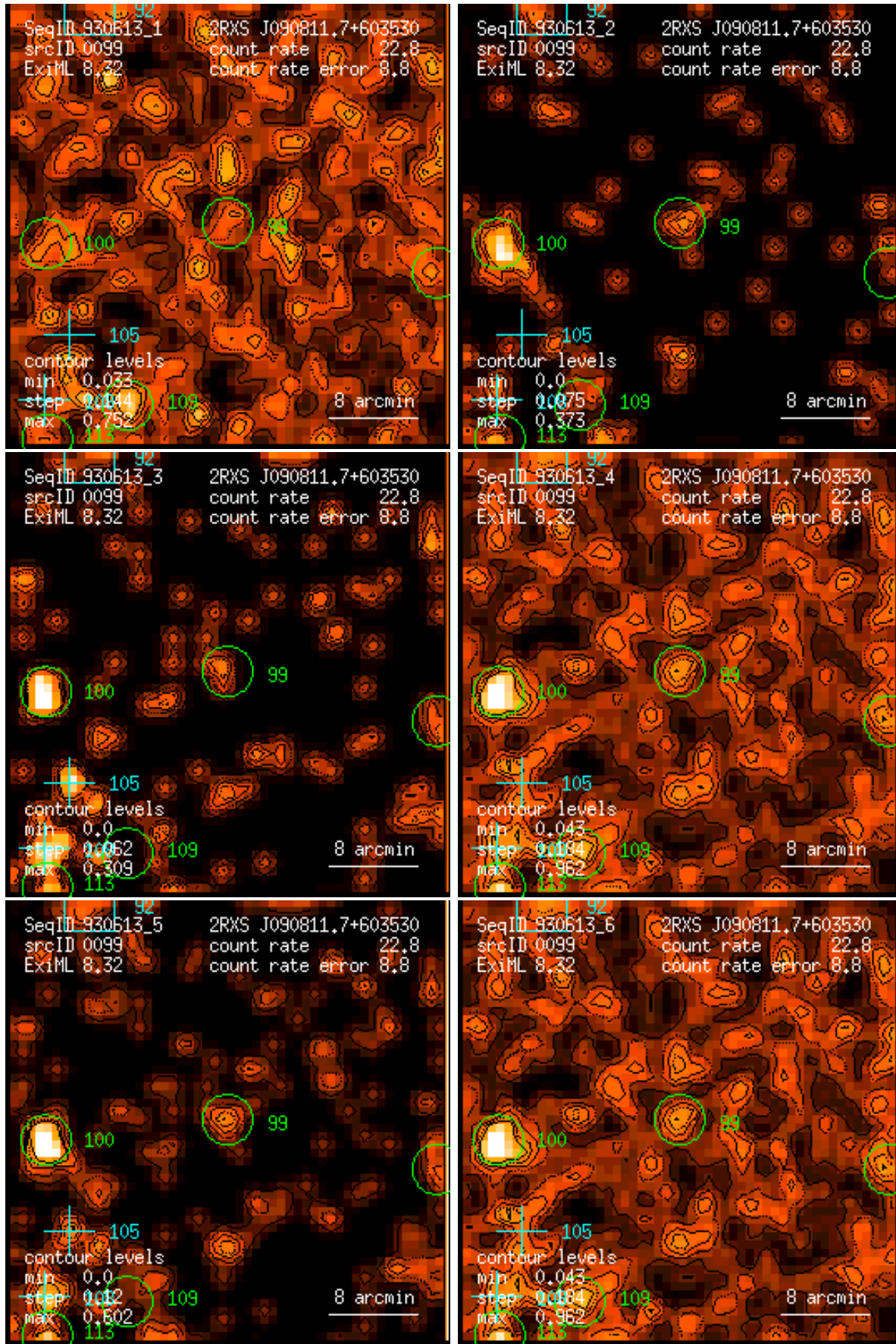
Figure 99: RASS 930613: detection 0099: band rate images, Gaussian filter: (1) PSPC channels 11 – 41, (2) 52 – 90, (3) 91 – 201, (4) 11 – 235, (5) 52 – 201, (6) 11 – 201. Broad band rates in counts/ks. Band rate contour levels in counts/ks/arcmin 2 .
