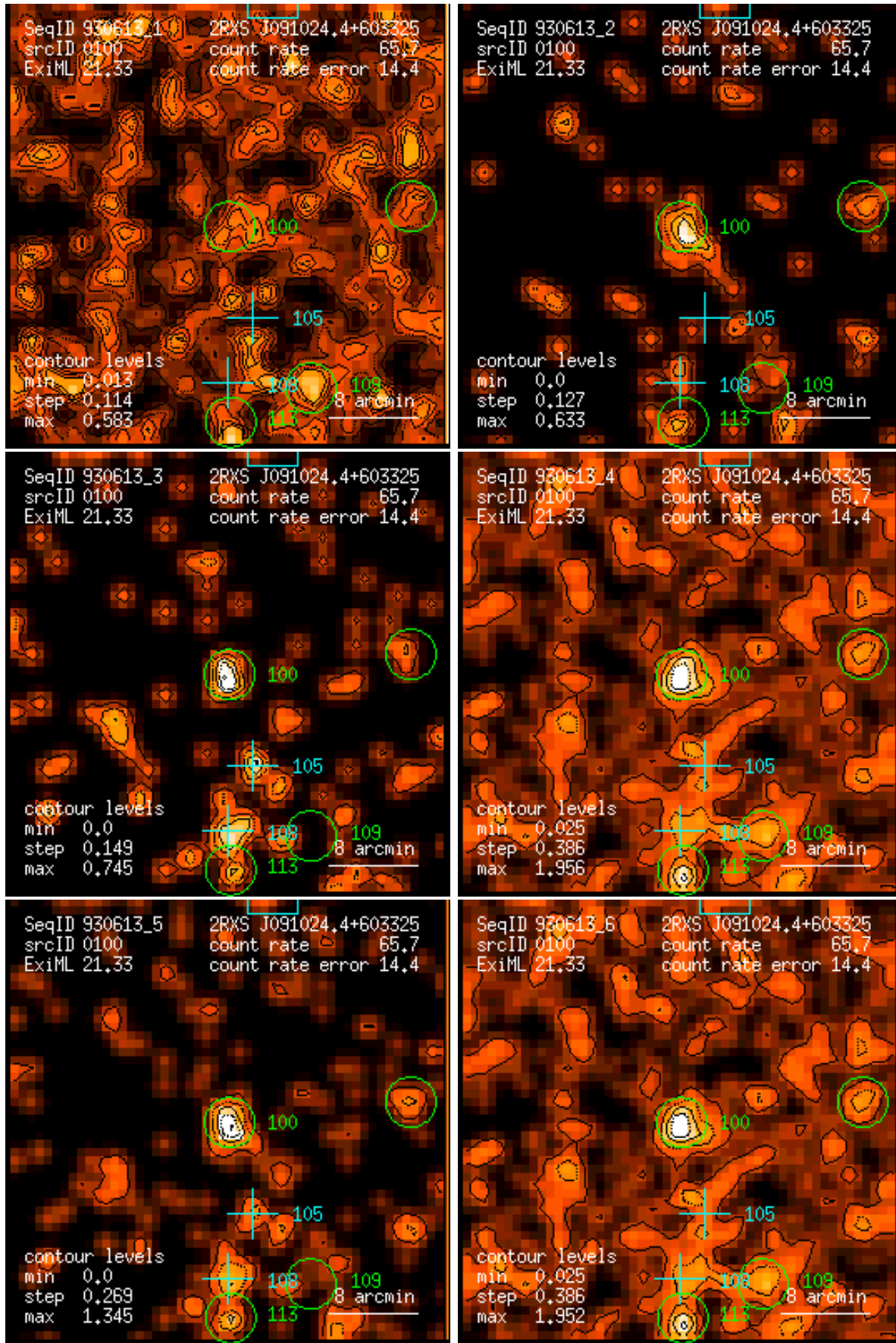
Figure 100: RASS 930613: detection 0100: band rate images, Gaussian filter: (1) PSPC channels 11 – 41, (2) 52 – 90, (3) 91 – 201, (4) 11 – 235, (5) 52 – 201, (6) 11 – 201. Broad band rates in counts/ks. Band rate contour levels in counts/ks/arcmin 2 .
