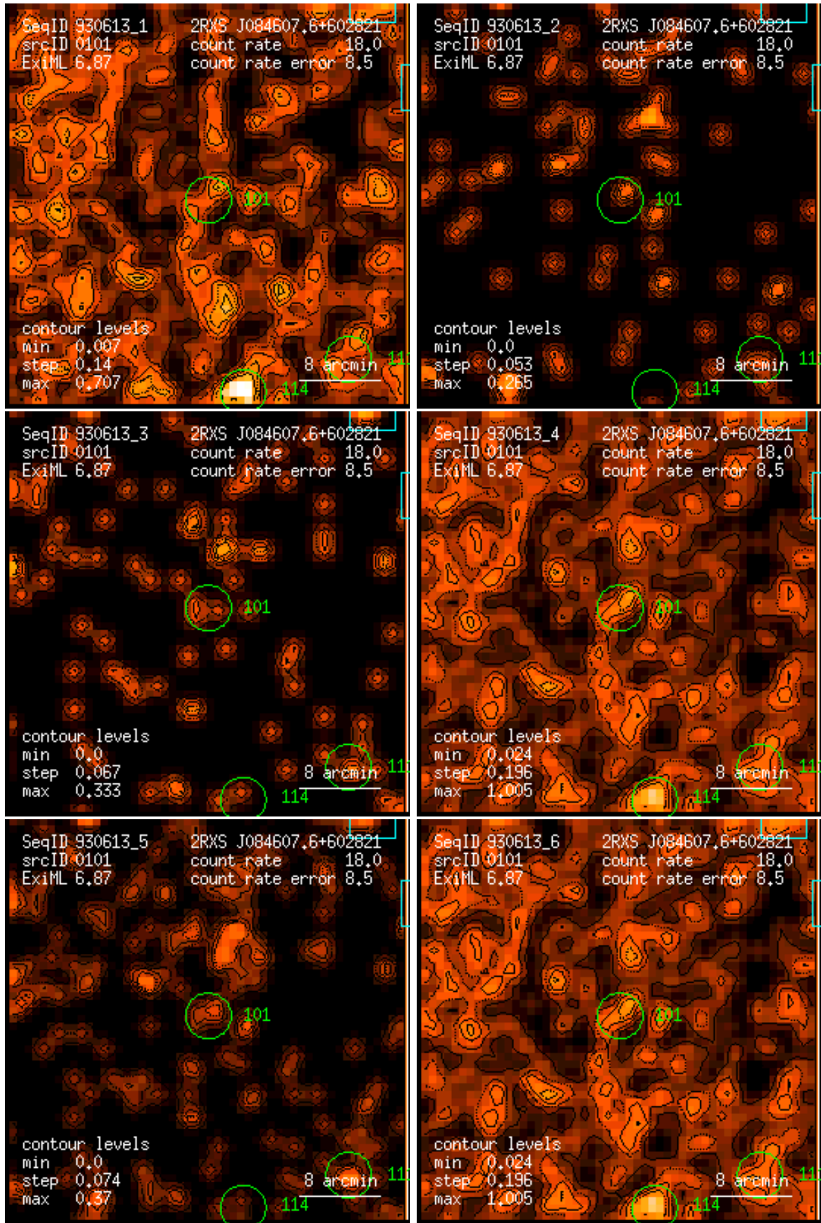
Figure 101: RASS 930613: detection 0101: band rate images, Gaussian filter: (1) PSPC channels 11 – 41, (2) 52 – 90, (3) 91 – 201, (4) 11 – 235, (5) 52 – 201, (6) 11 – 201. Broad band rates in counts/ks. Band rate contour levels in counts/ks/arcmin 2 .
