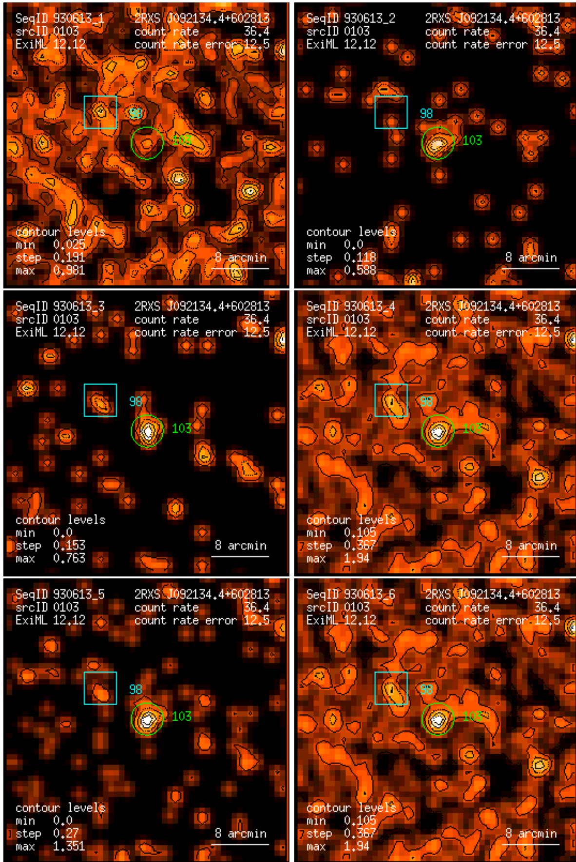
Figure 103: RASS 930613: detection 0103: band rate images, Gaussian filter: (1) PSPC channels 11 – 41, (2) 52 – 90, (3) 91 – 201, (4) 11 – 235, (5) 52 – 201, (6) 11 – 201. Broad band rates in counts/ks. Band rate contour levels in counts/ks/arcmin 2 .
