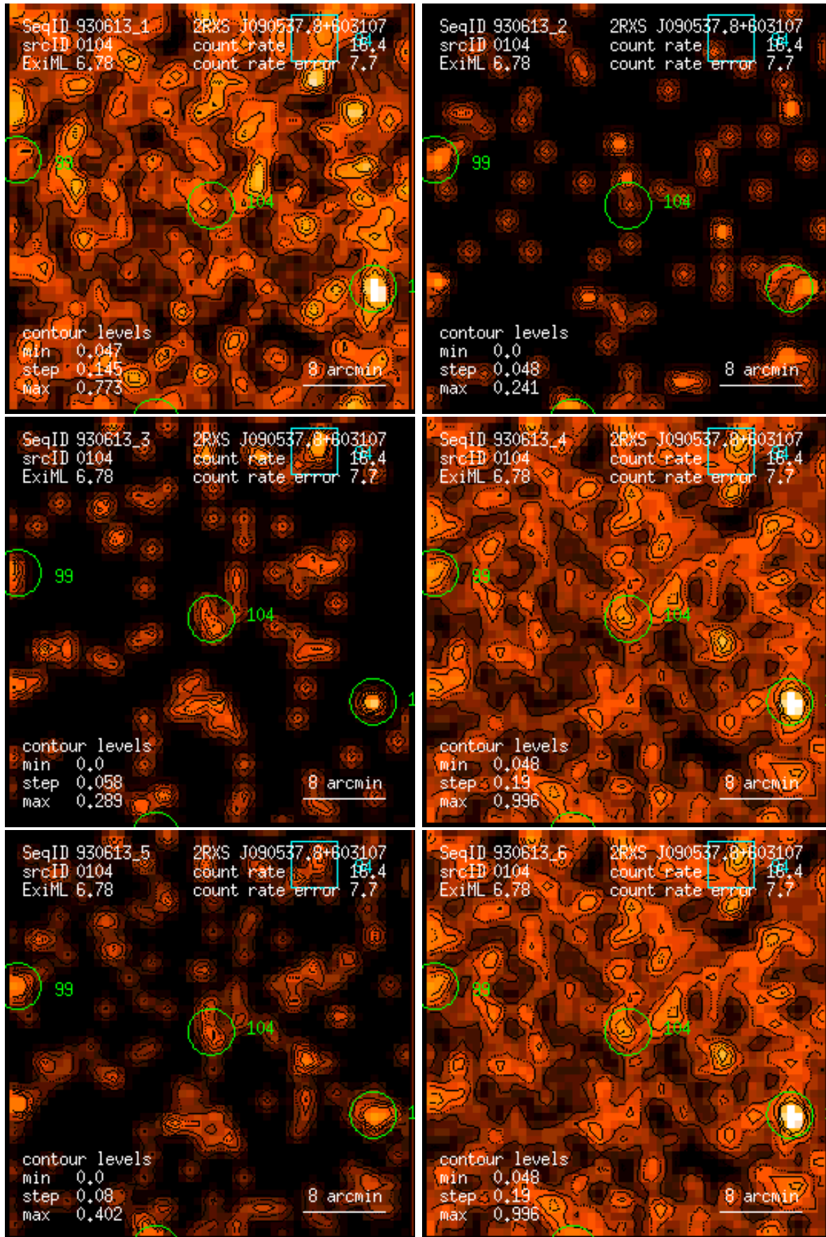
Figure 104: RASS 930613: detection 0104: band rate images, Gaussian filter: (1) PSPC channels 11 – 41, (2) 52 – 90, (3) 91 – 201, (4) 11 – 235, (5) 52 – 201, (6) 11 – 201. Broad band rates in counts/ks. Band rate contour levels in counts/ks/arcmin 2 .
