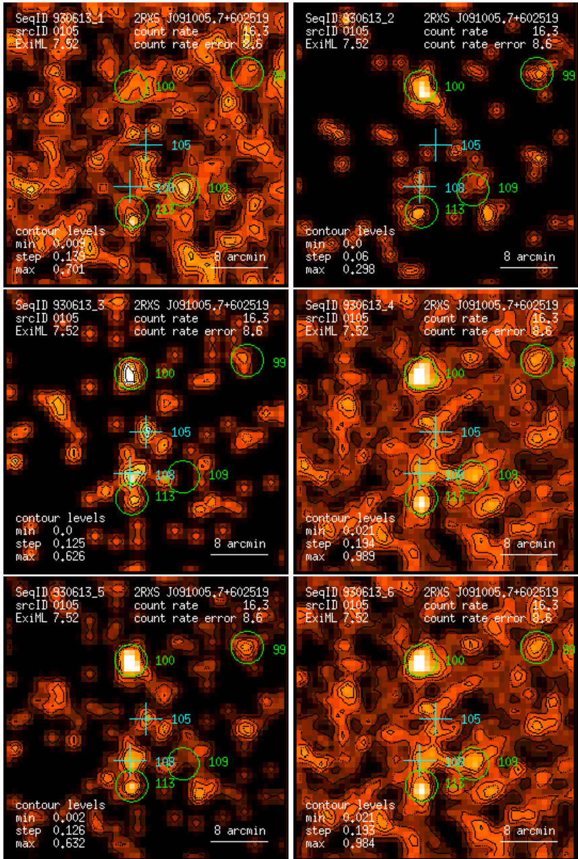
Figure 105: RASS 930613: detection 0105: band rate images, Gaussian filter: (1) PSPC channels 11 – 41, (2) 52 – 90, (3) 91 – 201, (4) 11 – 235, (5) 52 – 201, (6) 11 – 201. Broad band rates in counts/ks. Band rate contour levels in counts/ks/arcmin 2 .
