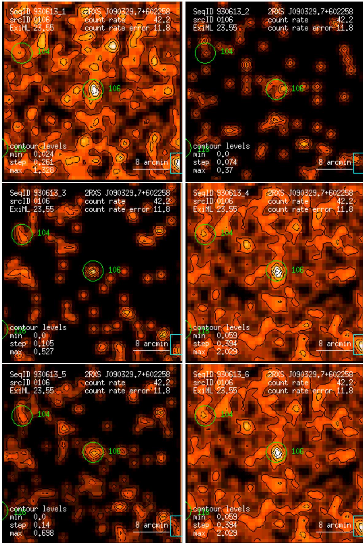
Figure 106: RASS 930613: detection 0106: band rate images, Gaussian filter: (1) PSPC channels 11 – 41, (2) 52 – 90, (3) 91 – 201, (4) 11 – 235, (5) 52 – 201, (6) 11 – 201. Broad band rates in counts/ks. Band rate contour levels in counts/ks/arcmin 2 .
