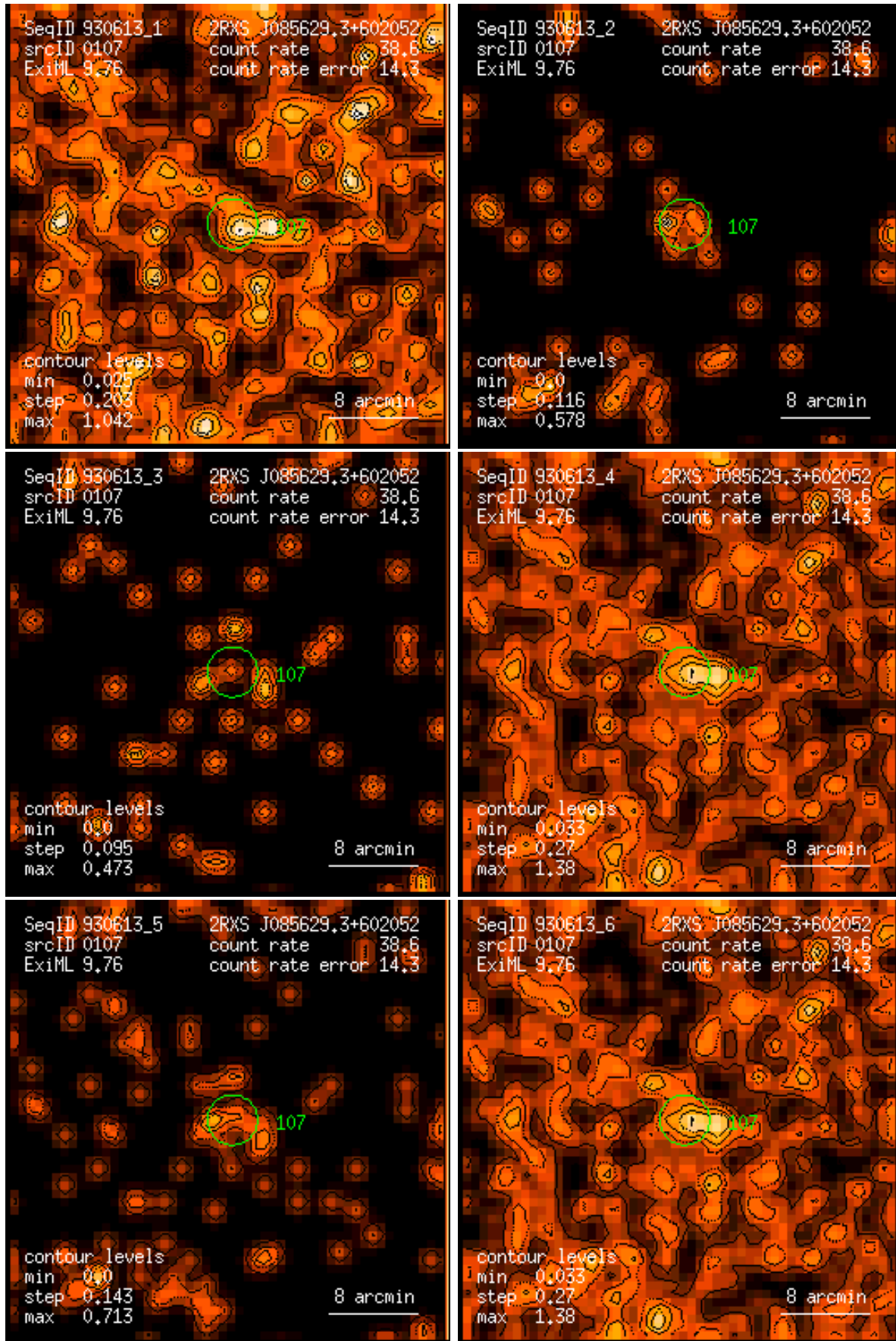
Figure 107: RASS 930613: detection 0107: band rate images, Gaussian filter: (1) PSPC channels 11 – 41, (2) 52 – 90, (3) 91 – 201, (4) 11 – 235, (5) 52 – 201, (6) 11 – 201. Broad band rates in counts/ks. Band rate contour levels in counts/ks/arcmin 2 .
