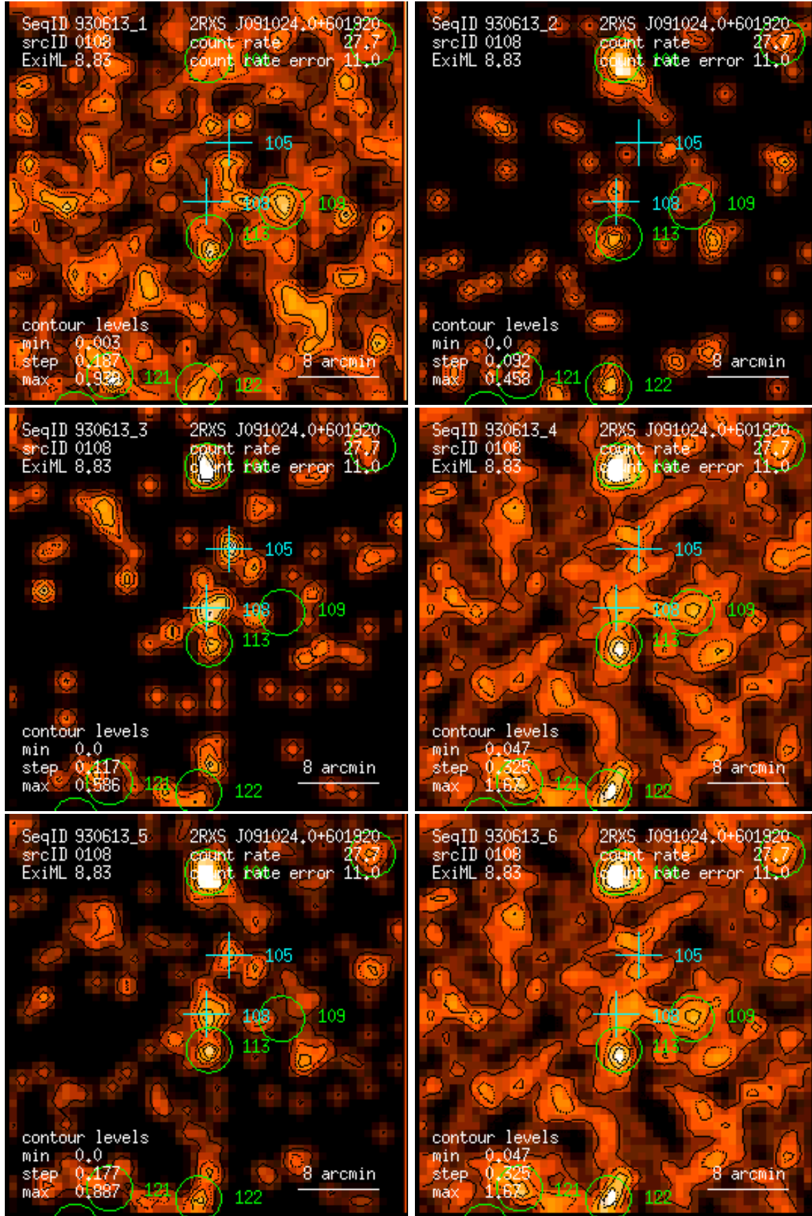
Figure 108: RASS 930613: detection 0108: band rate images, Gaussian filter: (1) PSPC channels 11 – 41, (2) 52 – 90, (3) 91 – 201, (4) 11 – 235, (5) 52 – 201, (6) 11 – 201. Broad band rates in counts/ks. Band rate contour levels in counts/ks/arcmin 2 .
