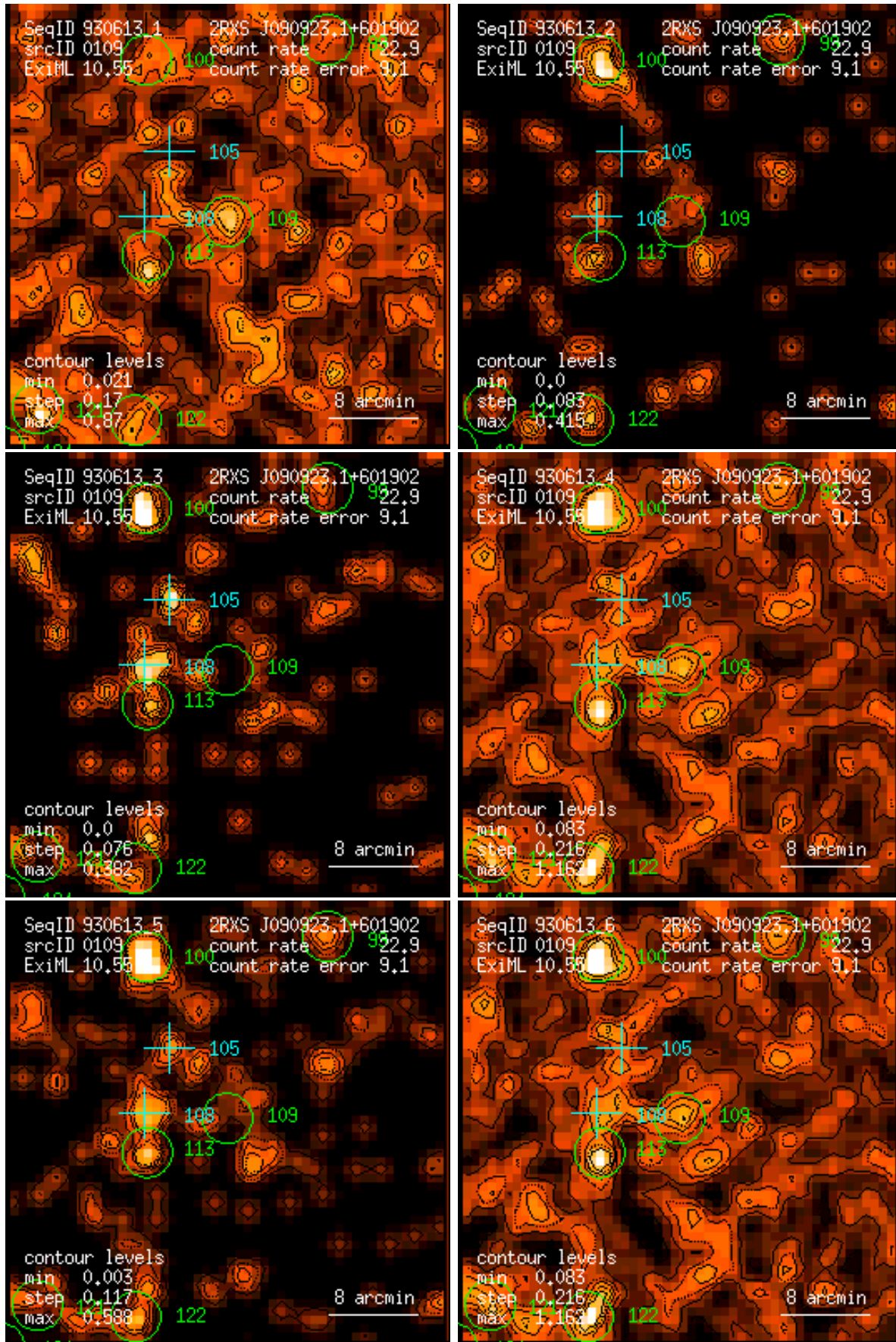
Figure 109: RASS 930613: detection 0109: band rate images, Gaussian filter: (1) PSPC channels 11 – 41, (2) 52 – 90, (3) 91 – 201, (4) 11 – 235, (5) 52 – 201, (6) 11 – 201. Broad band rates in counts/ks. Band rate contour levels in counts/ks/arcmin 2 .
