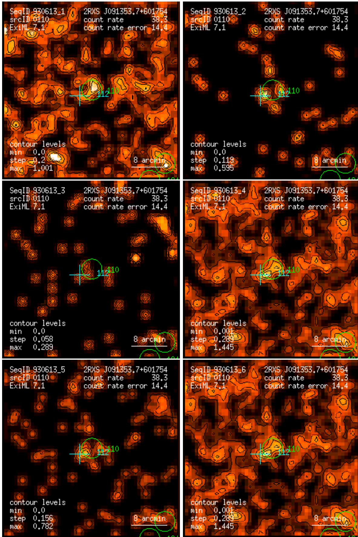
Figure 110: RASS 930613: detection 0110: band rate images, Gaussian filter: (1) PSPC channels 11 – 41, (2) 52 – 90, (3) 91 – 201, (4) 11 – 235, (5) 52 – 201, (6) 11 – 201. Broad band rates in counts/ks. Band rate contour levels in counts/ks/arcmin 2 .
